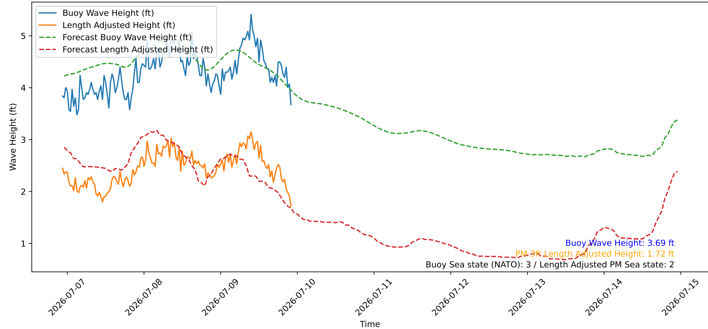
Wave Heights over Time for Oceanside Harbor at 2026-07-09 22:40:25
