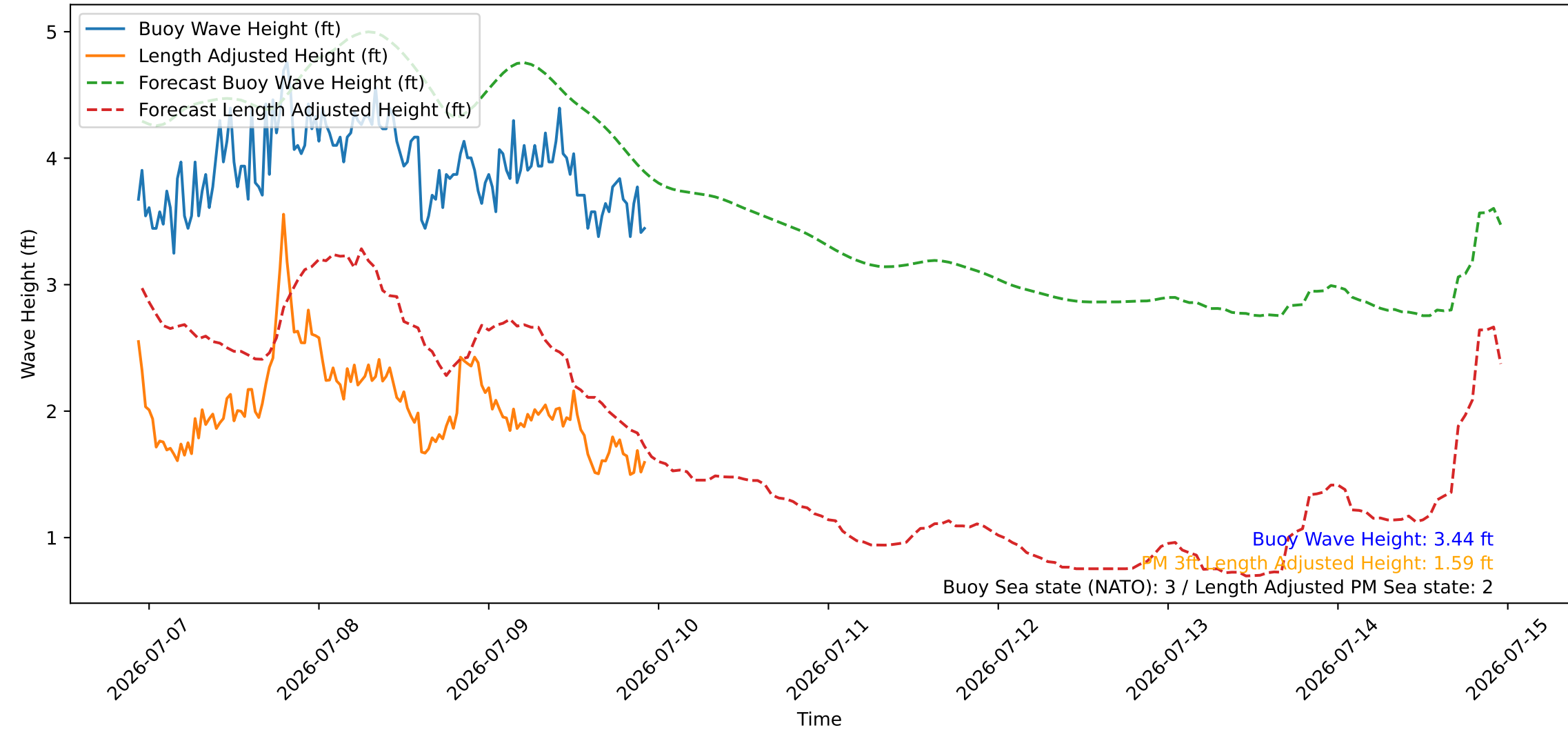
Wave Heights over Time for Green Beach at 2026-07-09 22:41:07
