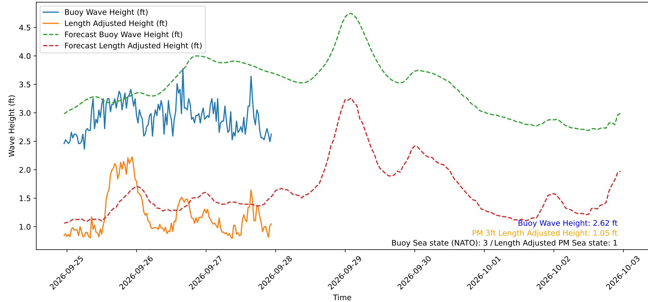
Wave Heights over Time for Oceanside Harbor at 2026-09-27 23:00:29
