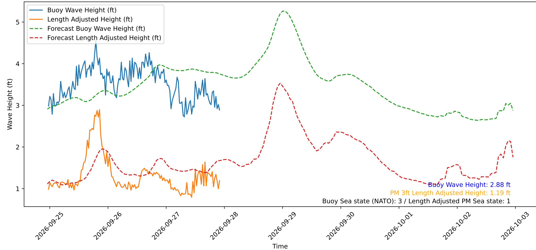
Wave Heights over Time for Green Beach at 2026-09-27 23:01:12
