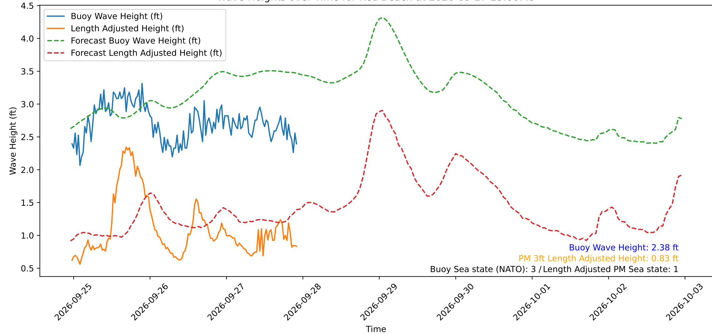
Wave Heights over Time for Red Beach at 2026-09-27 23:00:49
