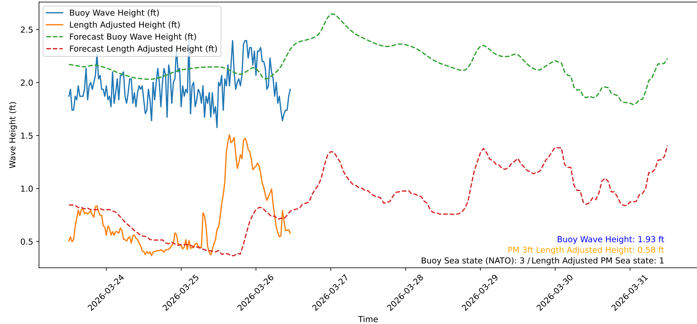
Wave Heights over Time for Red Beach at 2026-03-26 11:50:47
