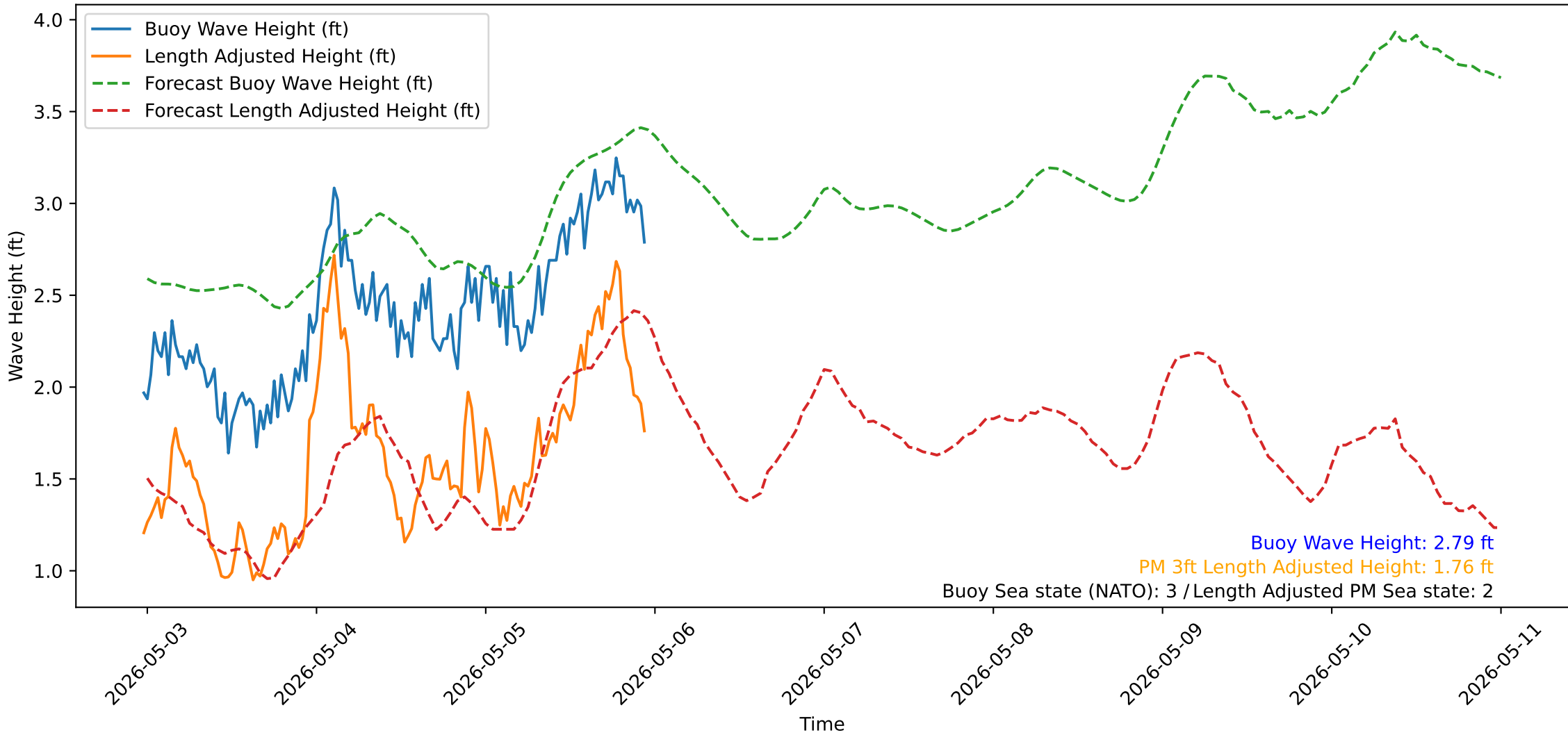
Wave Heights over Time for Oceanside Harbor at 2026-05-05 23:40:31
