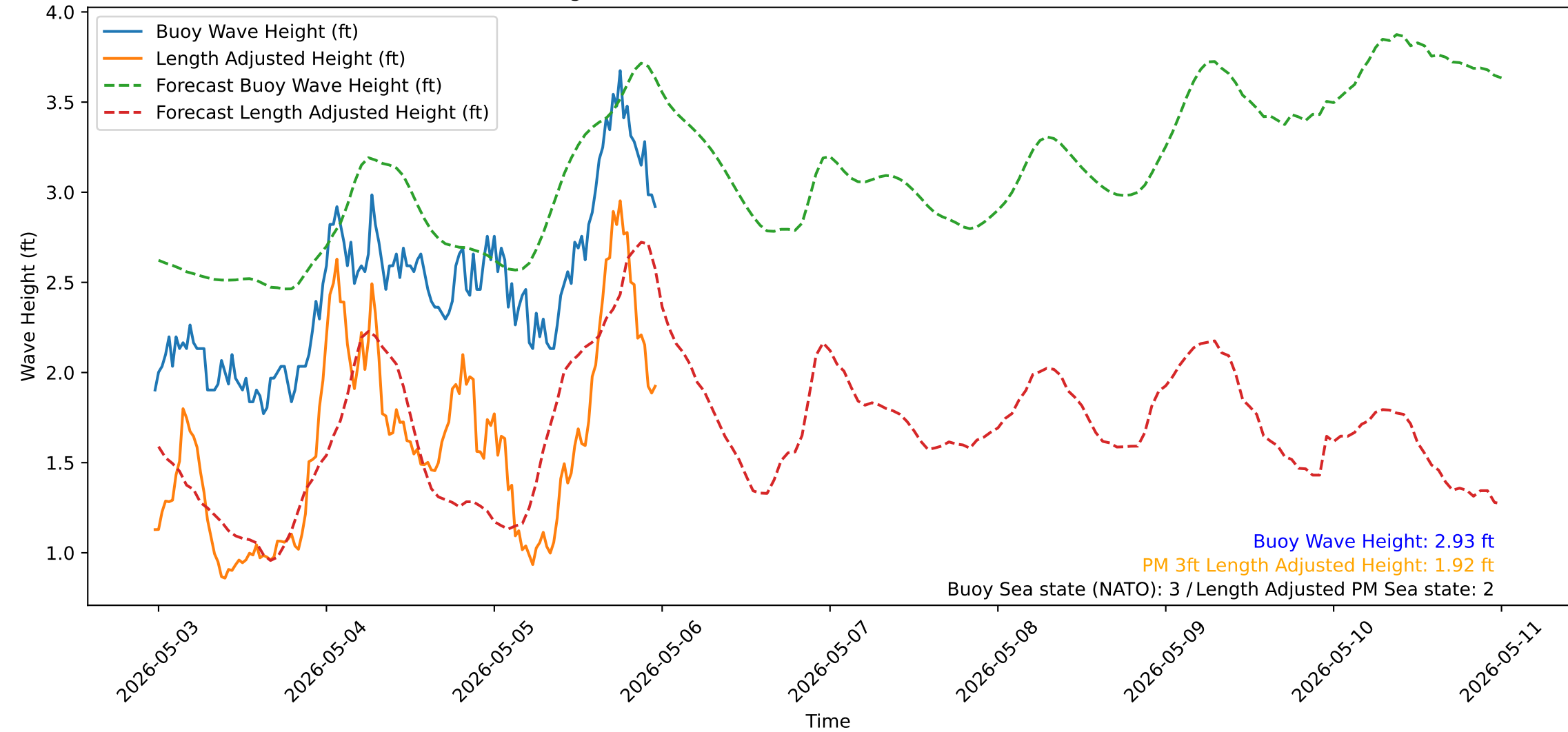
Wave Heights over Time for Green Beach at 2026-05-05 23:41:13
