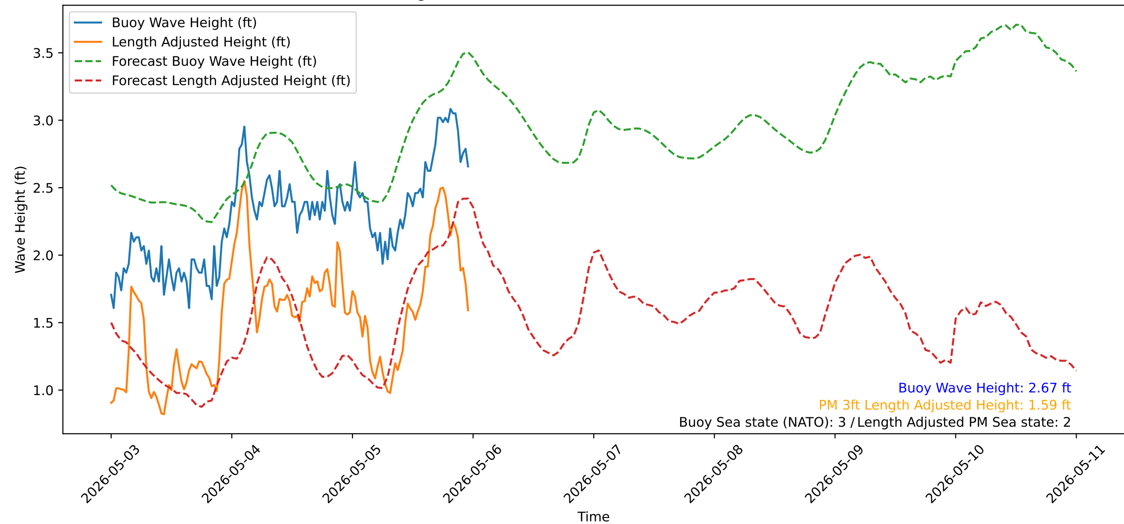
Wave Heights over Time for Red Beach at 2026-05-05 23:40:50
