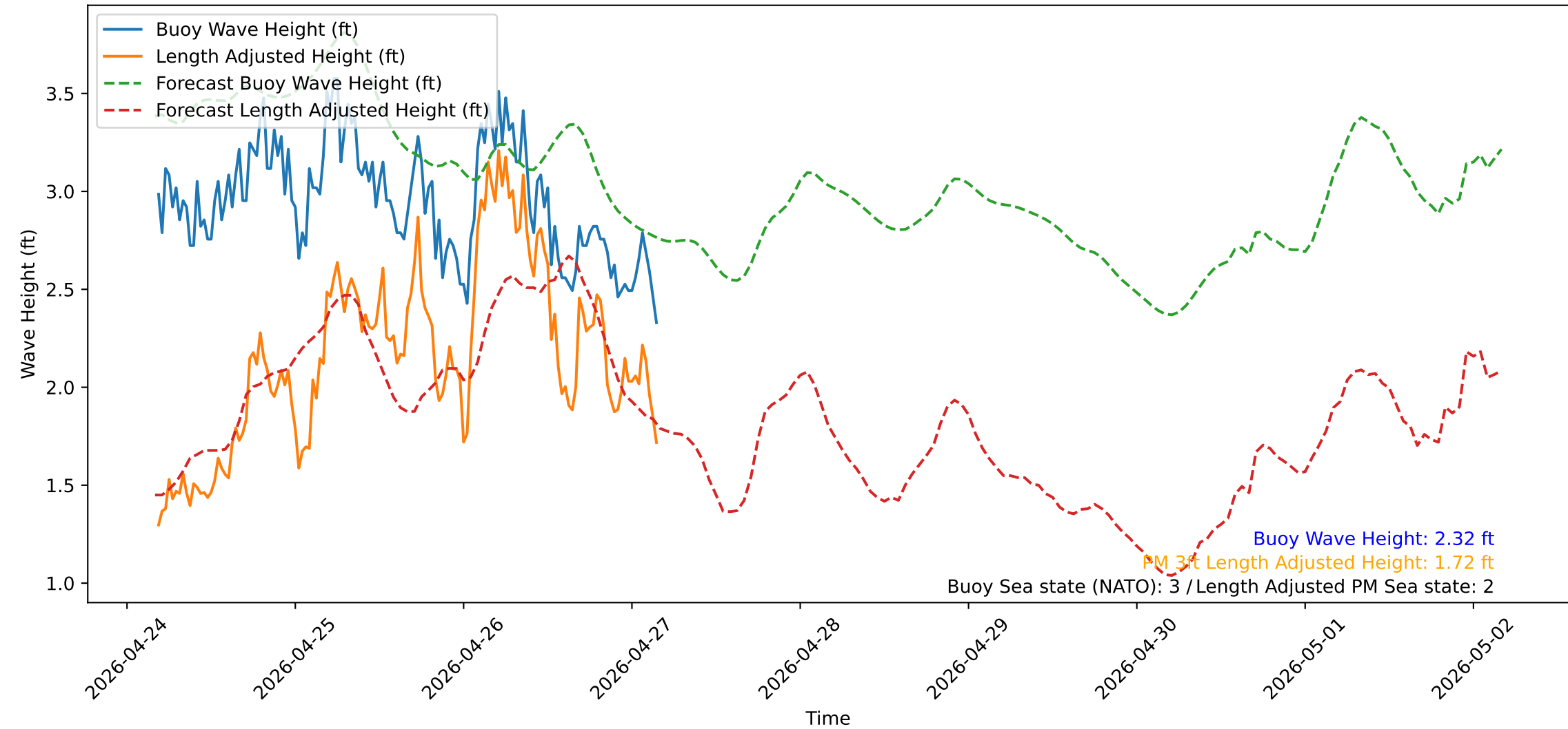
Wave Heights over Time for Green Beach at 2026-04-27 04:21:14
