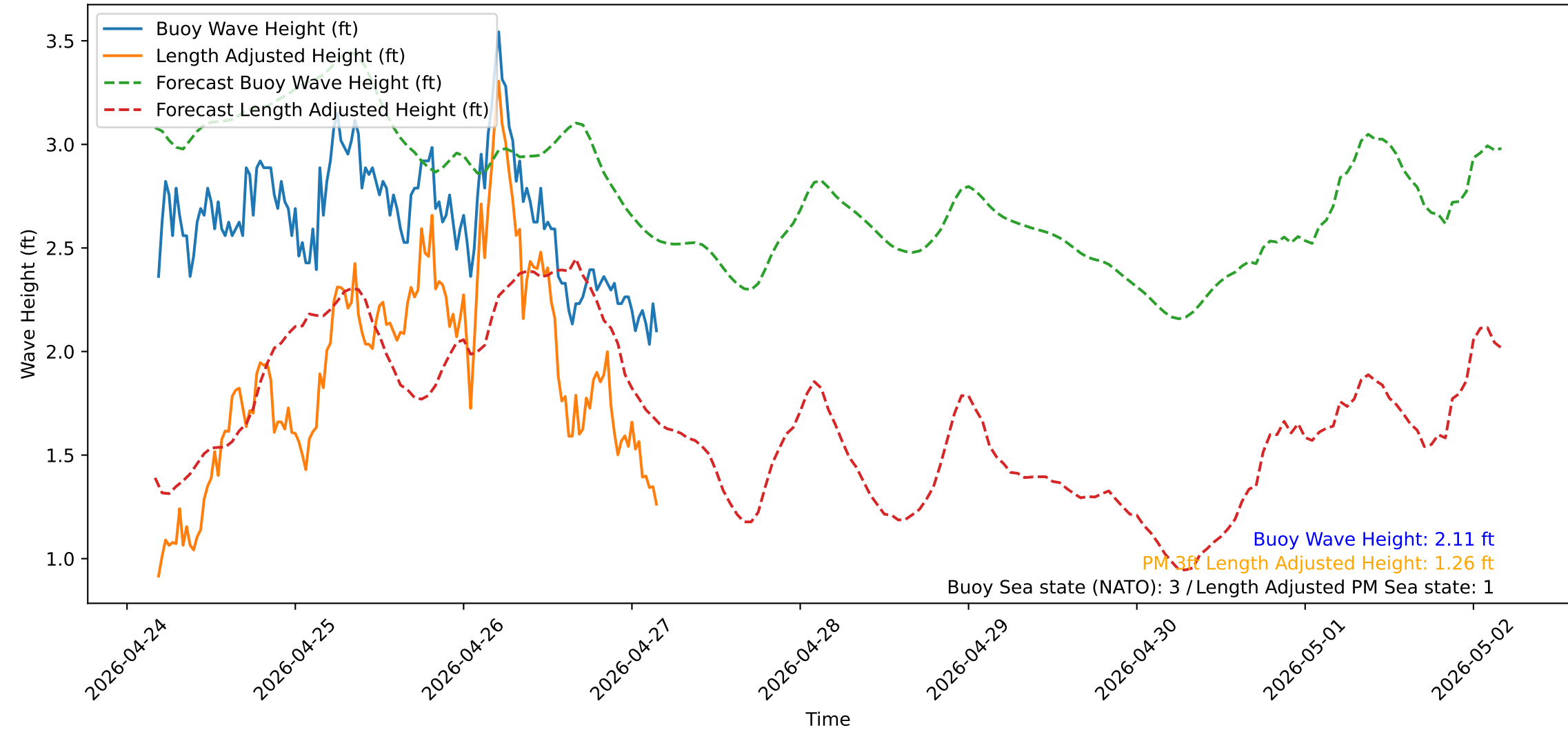
Wave Heights over Time for Red Beach at 2026-04-27 04:20:51
