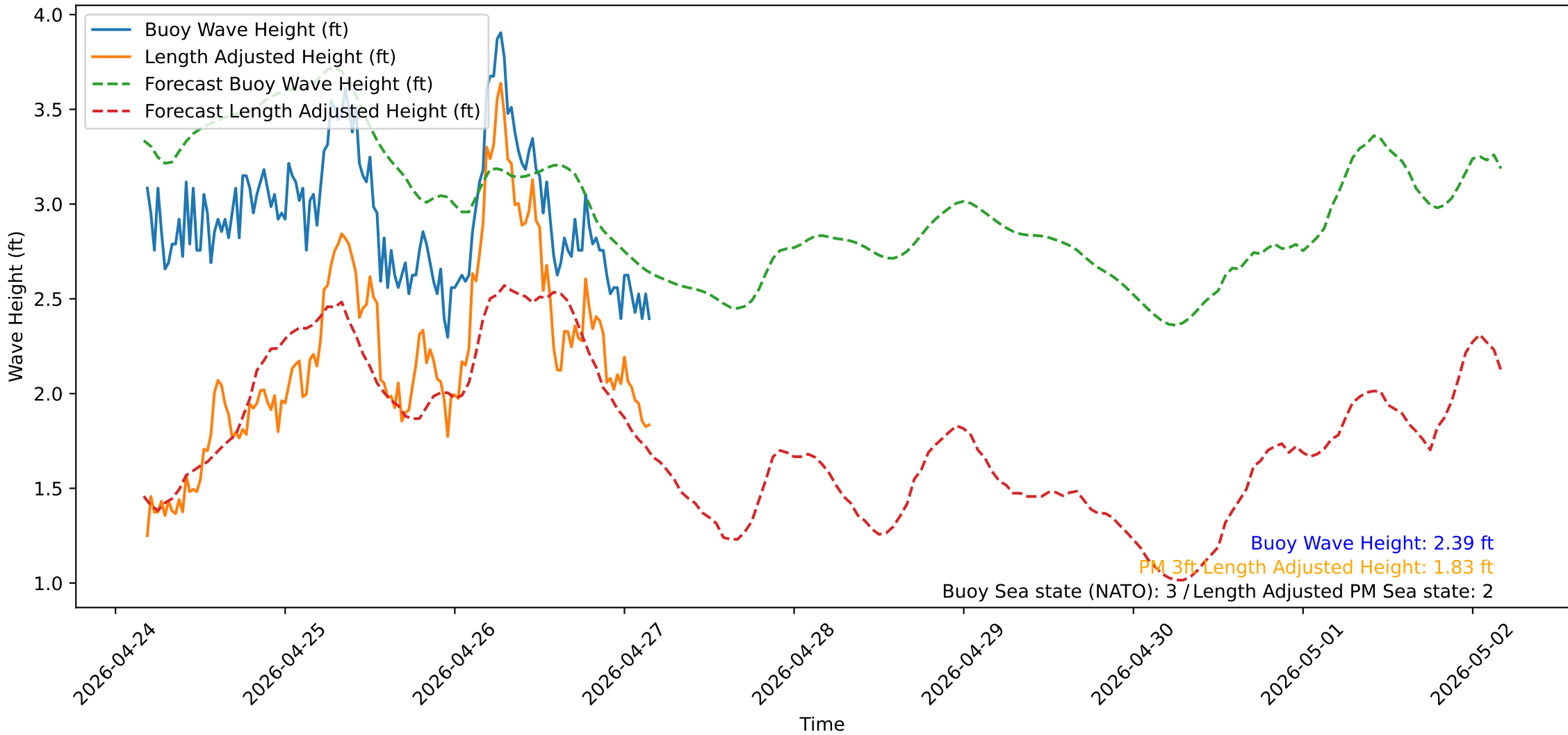
Wave Heights over Time for Oceanside Harbor at 2026-04-27 04:20:31
