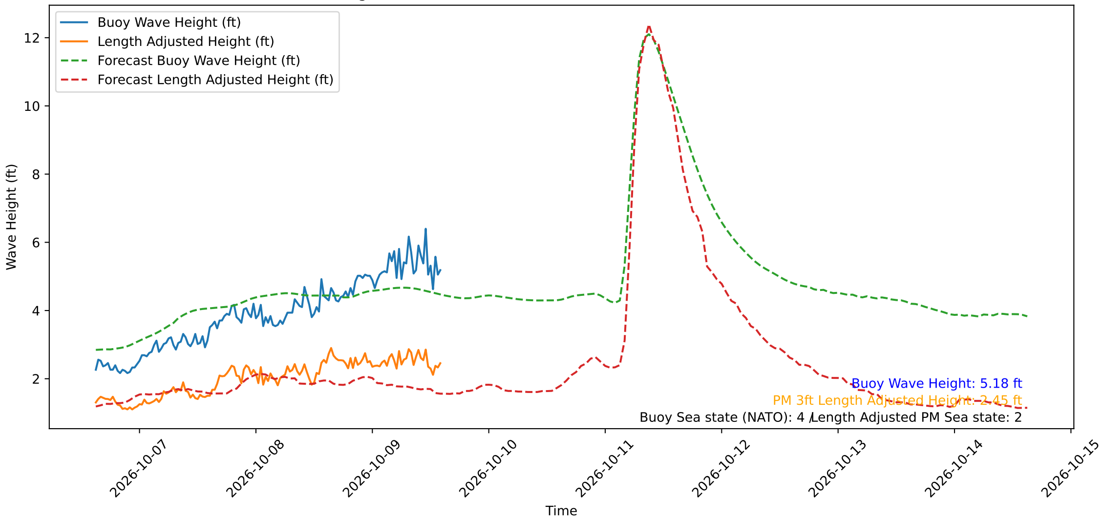
Wave Heights over Time for Oceanside Harbor at 2026-10-09 15:10:30
