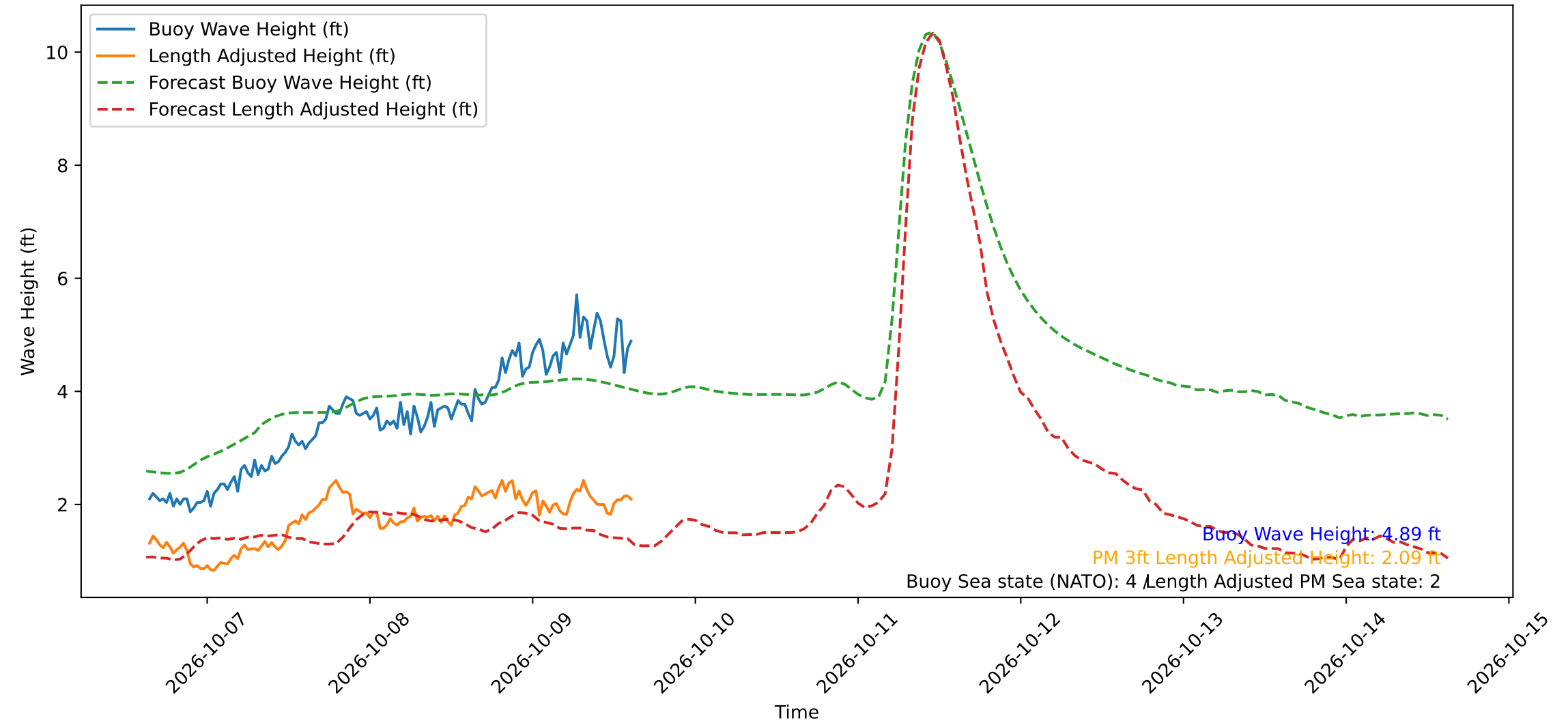
Wave Heights over Time for Red Beach at 2026-10-09 15:10:50
