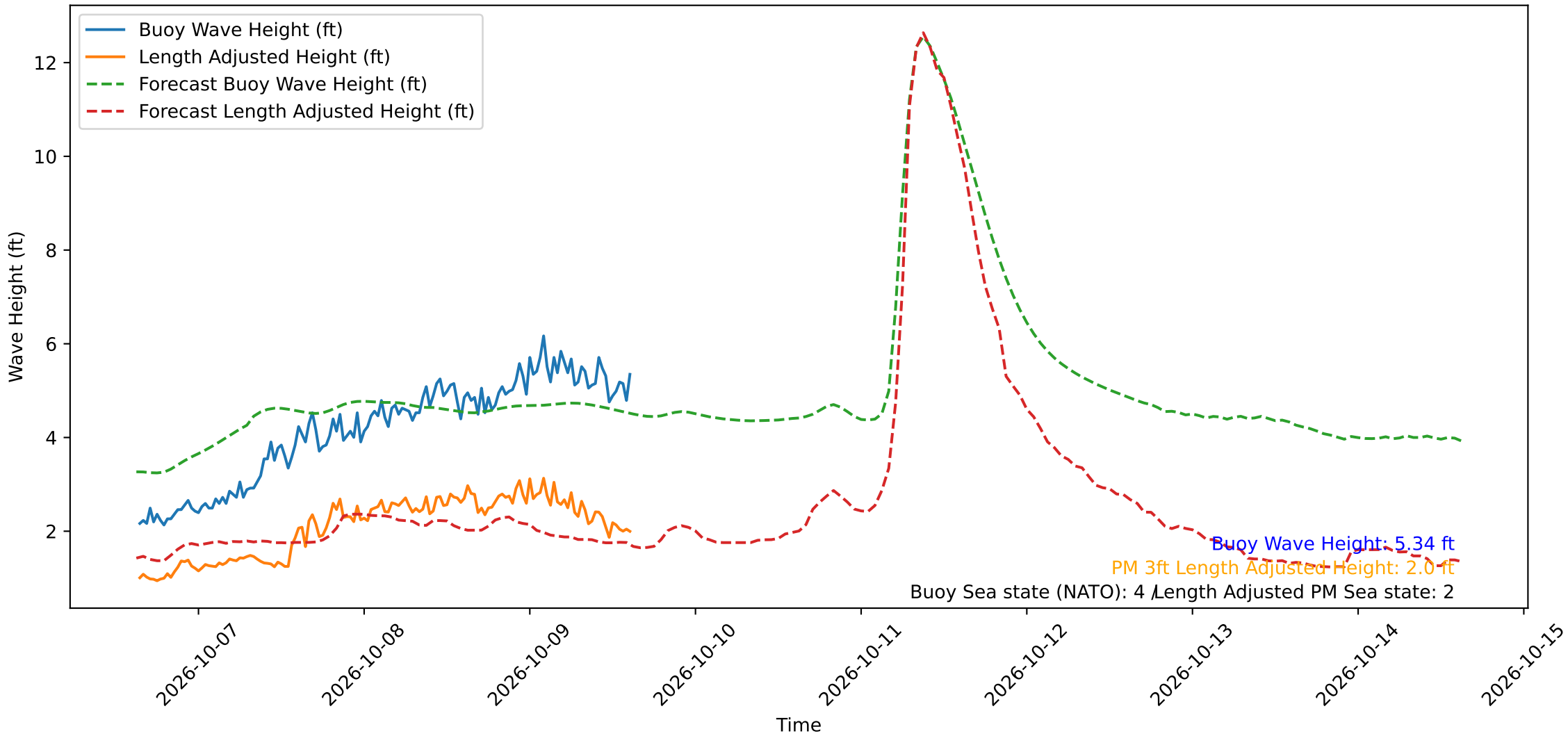
Wave Heights over Time for Green Beach at 2026-10-09 15:11:13
