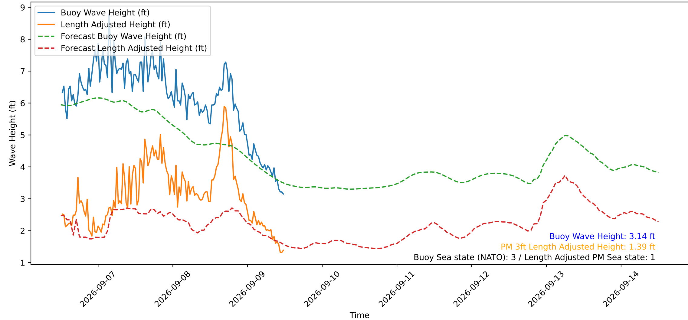
Wave Heights over Time for Green Beach at 2026-09-09 12:11:12
