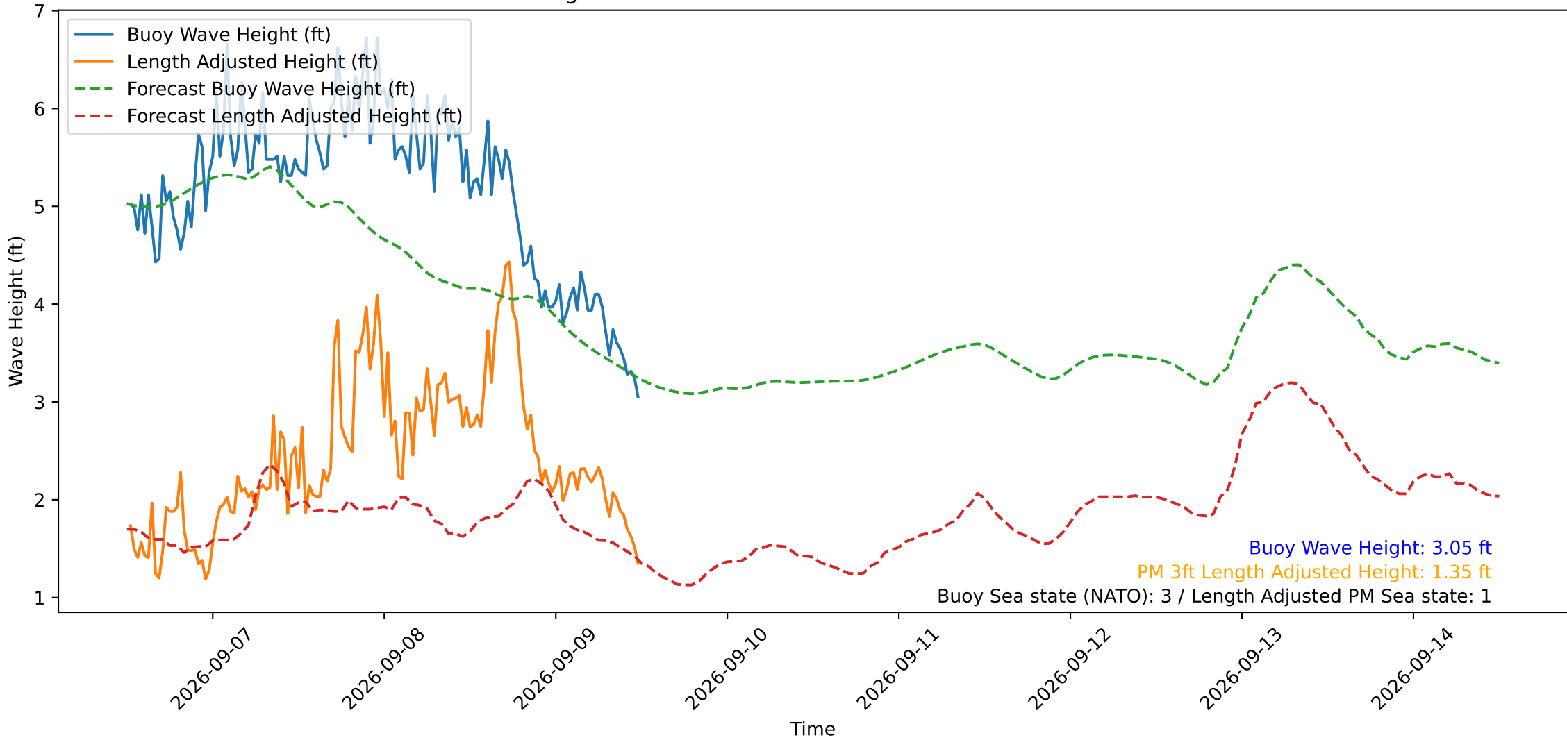
Wave Heights over Time for Red Beach at 2026-09-09 12:10:49
