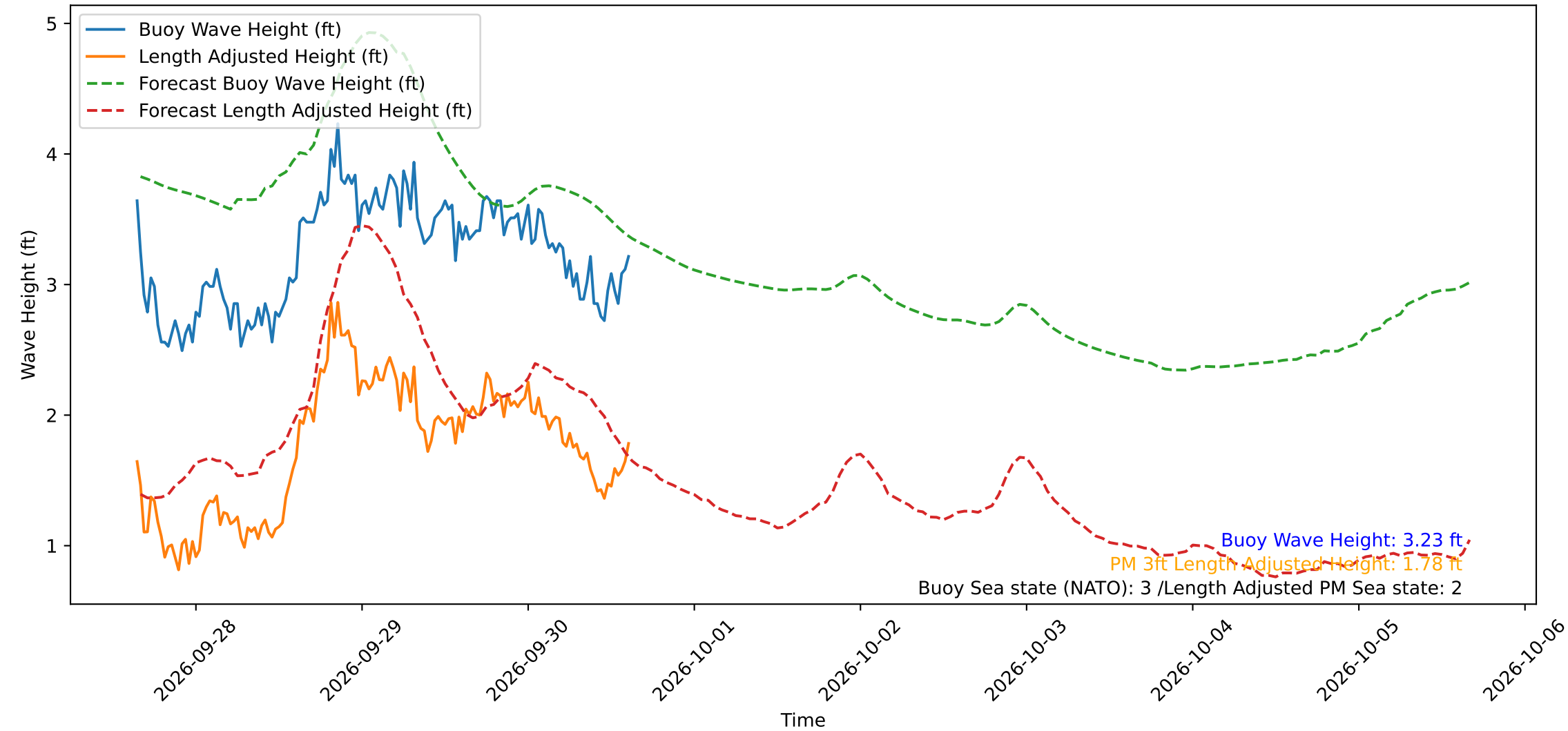
Wave Heights over Time for Oceanside Harbor at 2026-09-30 15:30:29
