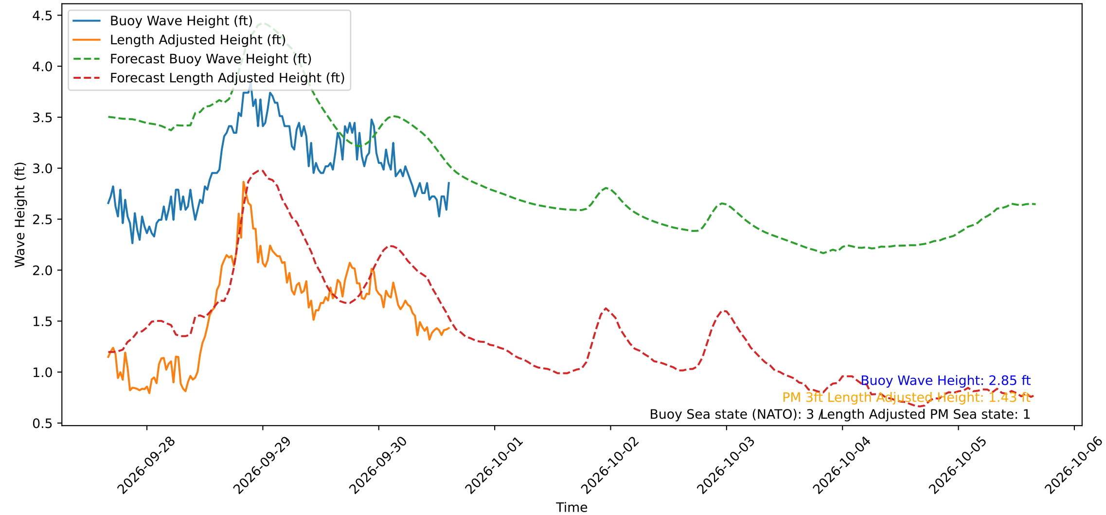
Wave Heights over Time for Red Beach at 2026-09-30 15:30:48
