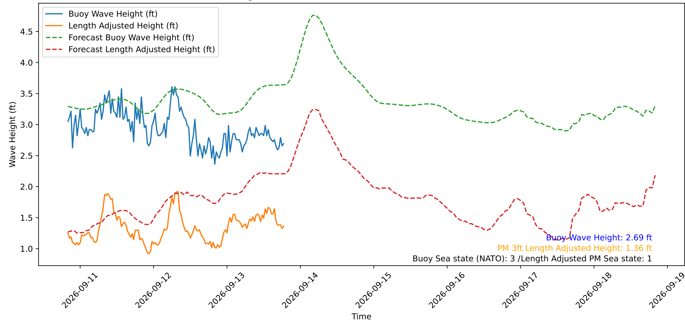
Wave Heights over Time for Green Beach at 2026-09-13 19:51:13
