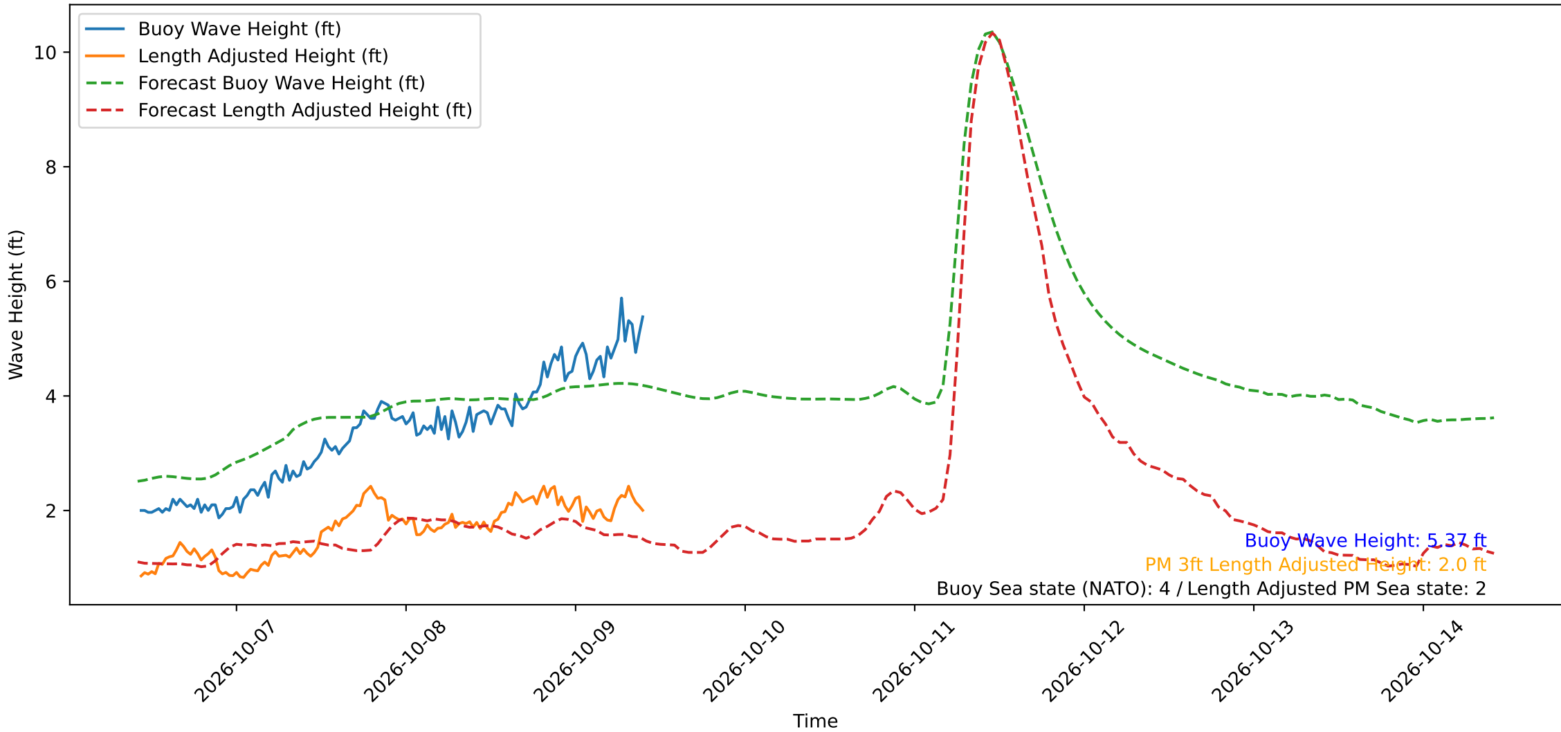
Wave Heights over Time for Red Beach at 2026-10-09 10:10:49
