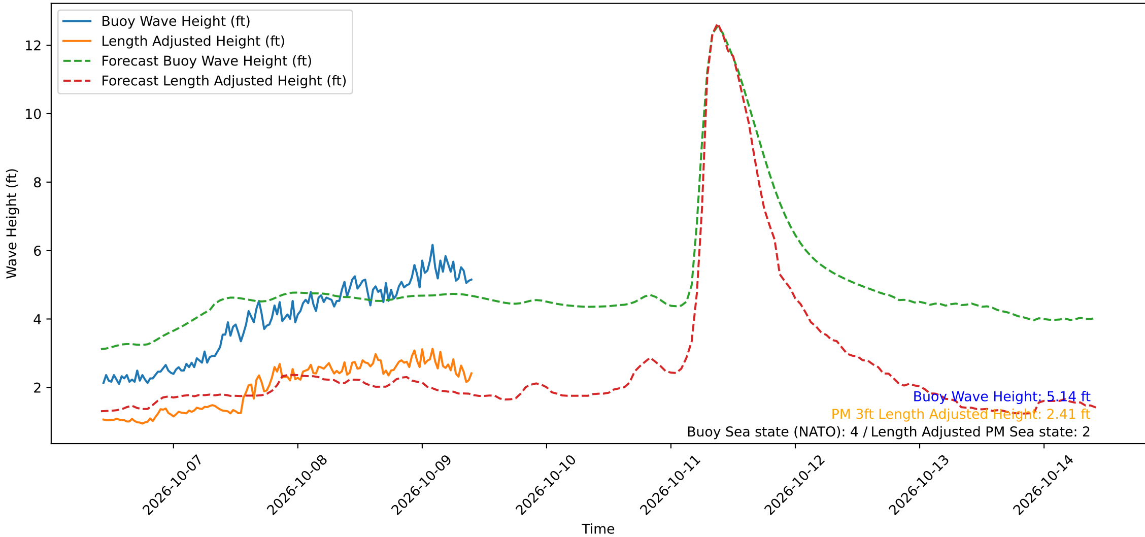
Wave Heights over Time for Green Beach at 2026-10-09 10:11:12
