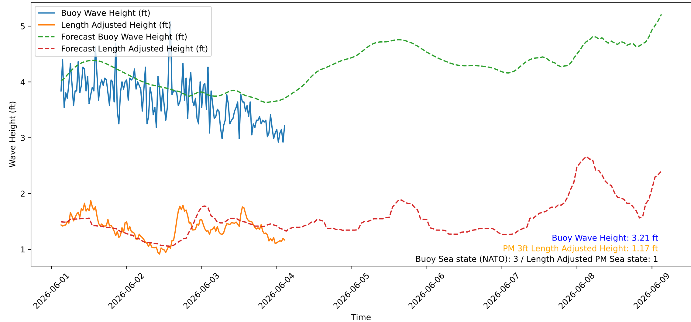
Wave Heights over Time for Oceanside Harbor at 2026-06-04 03:10:25
