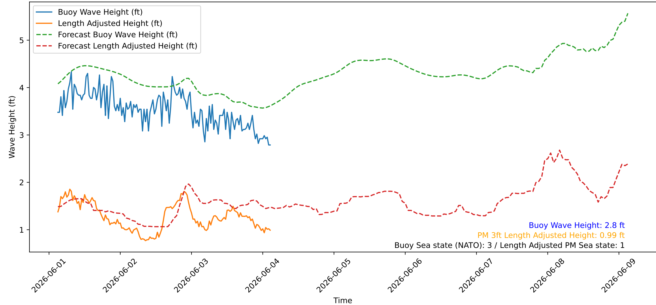
Wave Heights over Time for Green Beach at 2026-06-04 03:11:07
