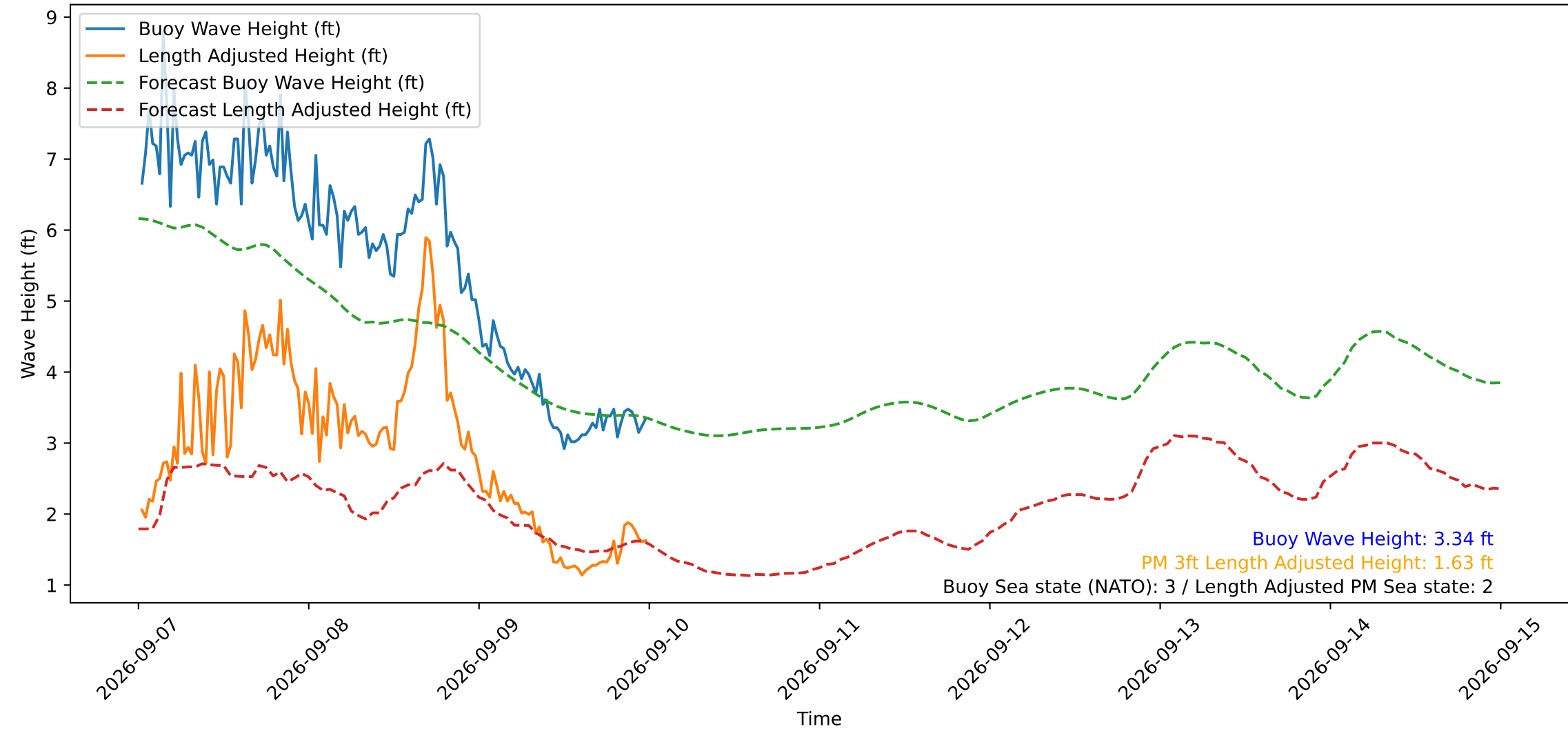
Wave Heights over Time for Green Beach at 2026-09-10 00:11:11
