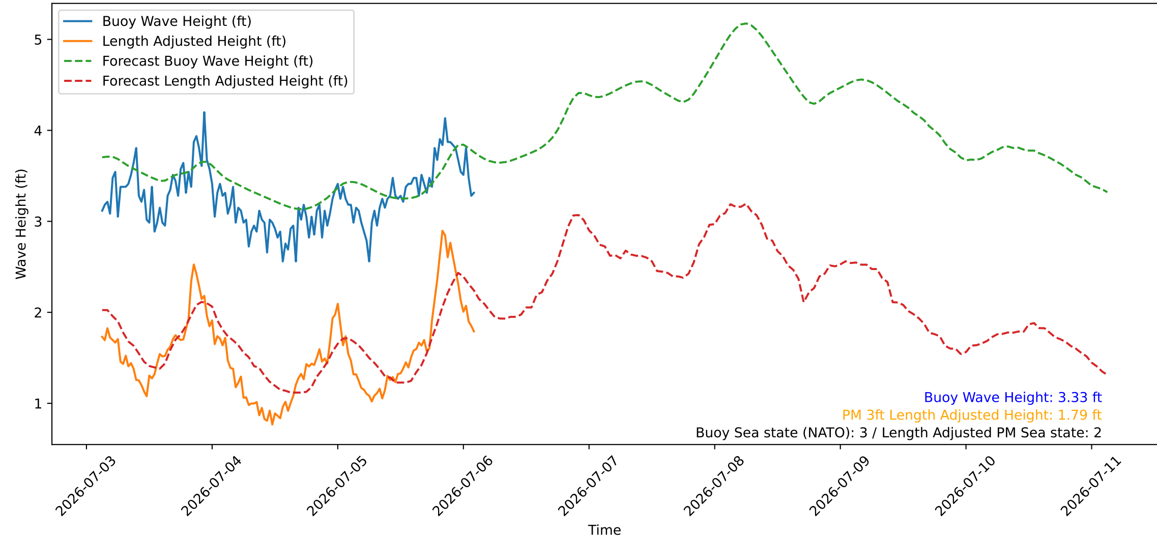
Wave Heights over Time for Green Beach at 2026-07-06 02:51:10
