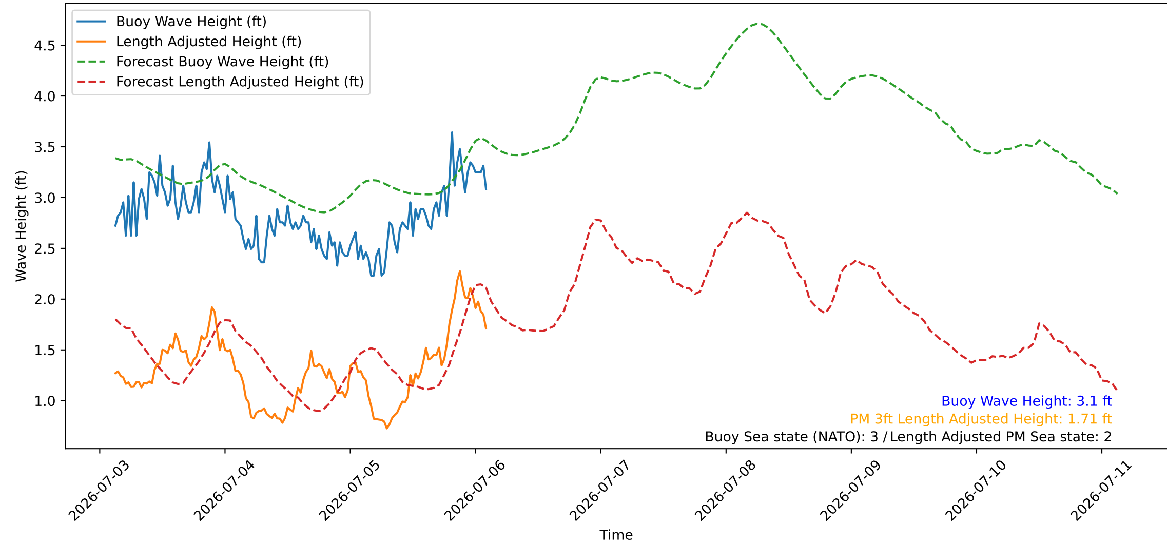
Wave Heights over Time for Red Beach at 2026-07-06 02:50:48
