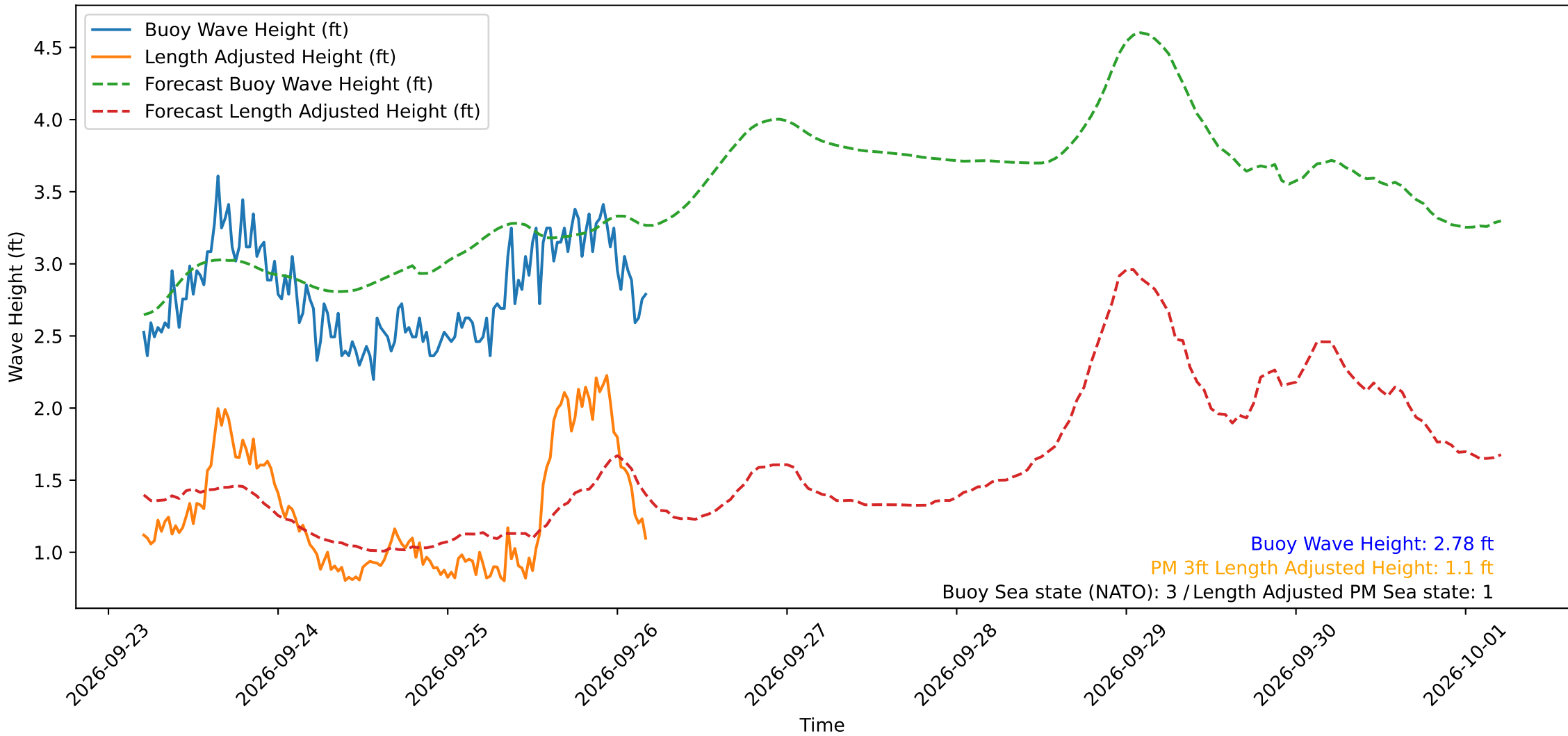
Wave Heights over Time for Oceanside Harbor at 2026-09-26 04:50:29
