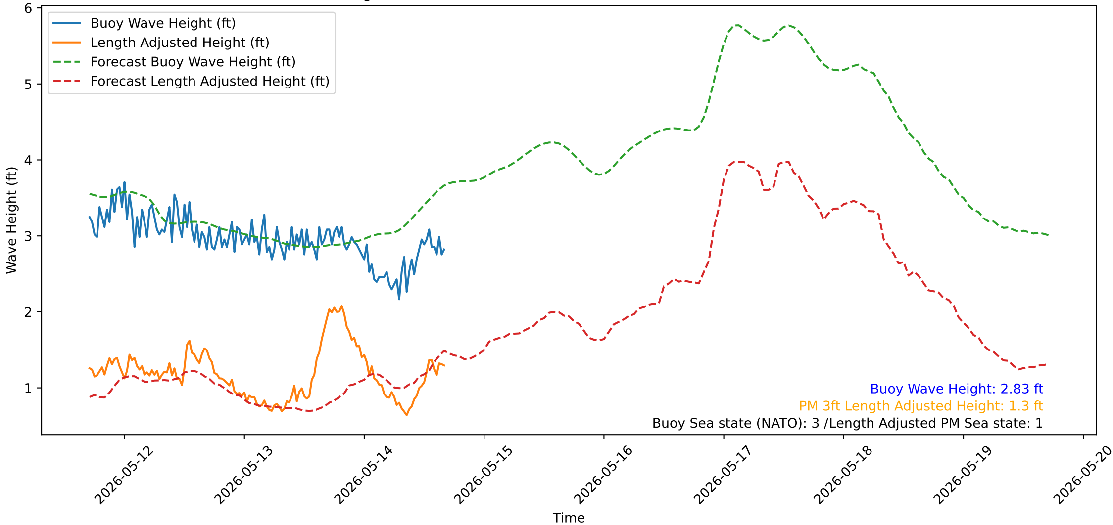
Wave Heights over Time for Oceanside Harbor at 2026-05-14 16:50:32
