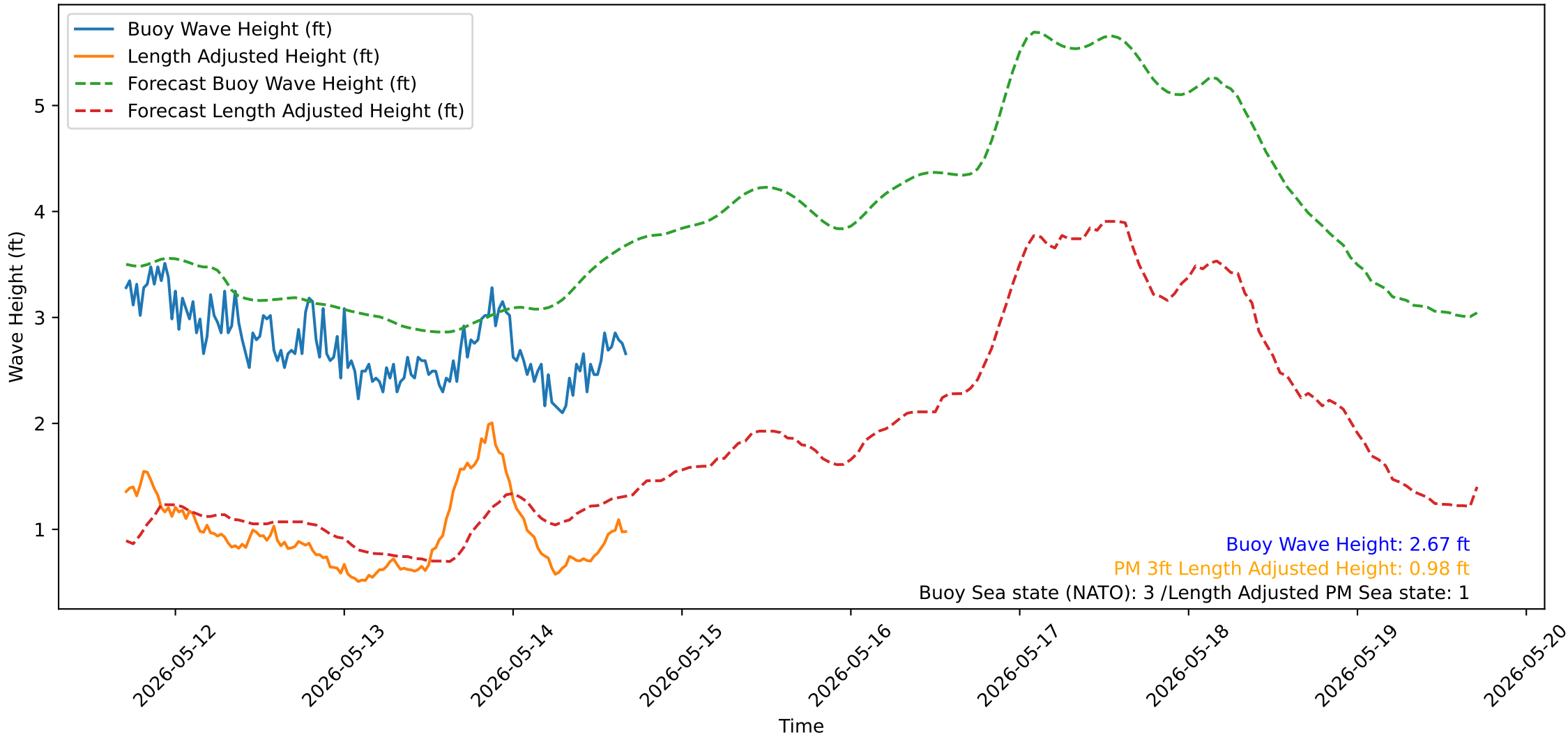
Wave Heights over Time for Green Beach at 2026-05-14 16:51:16
