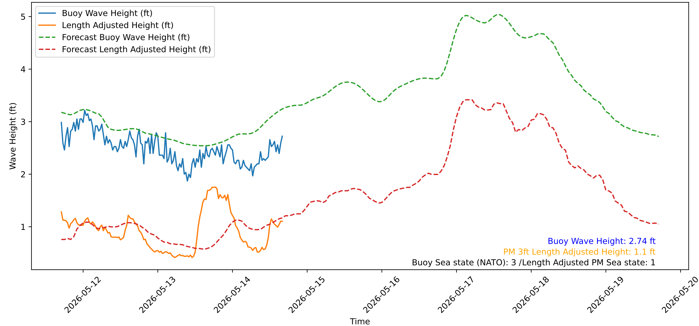
Wave Heights over Time for Red Beach at 2026-05-14 16:50:54
