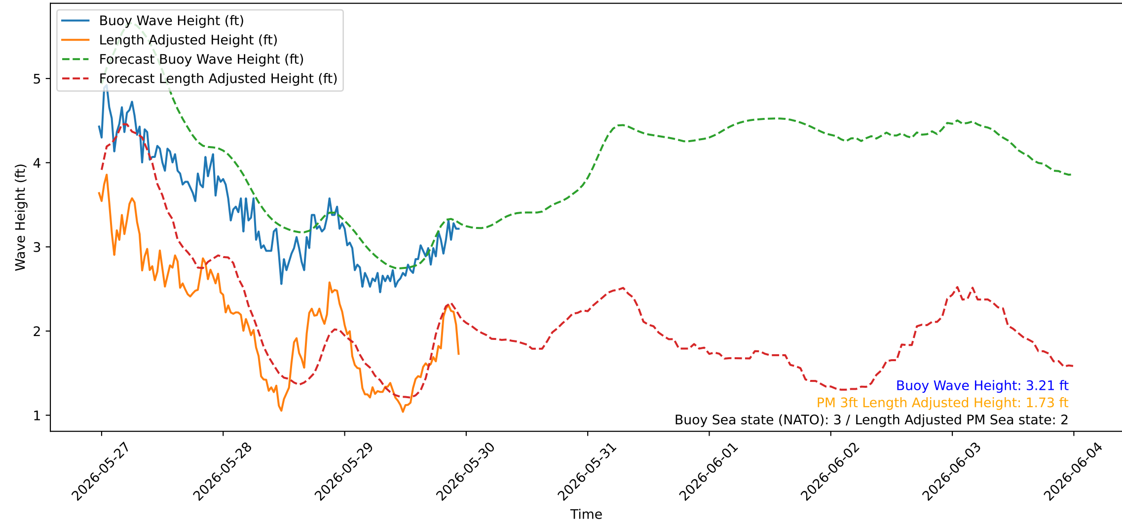
Wave Heights over Time for Green Beach at 2026-05-29 23:31:05
