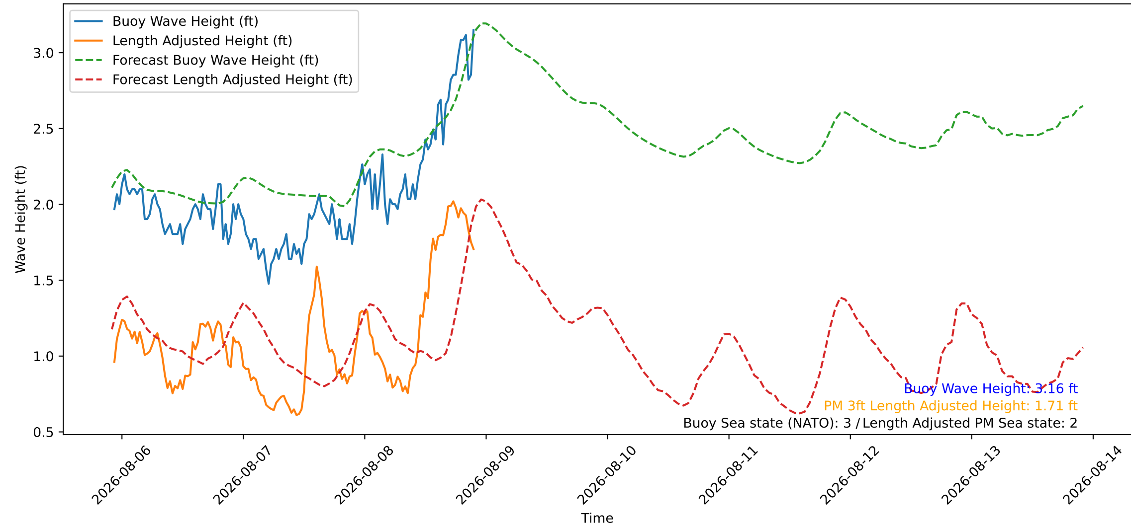
Wave Heights over Time for Red Beach at 2026-08-08 22:10:46
