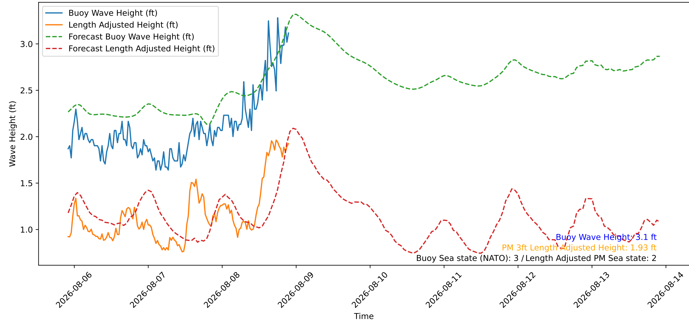
Wave Heights over Time for Oceanside Harbor at 2026-08-08 22:10:26
