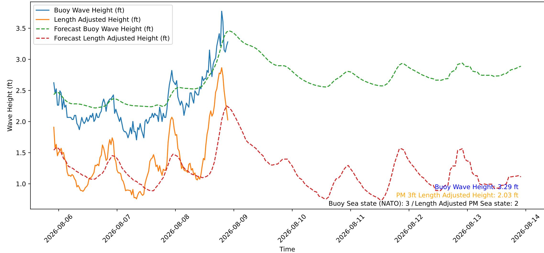
Wave Heights over Time for Green Beach at 2026-08-08 22:11:08
