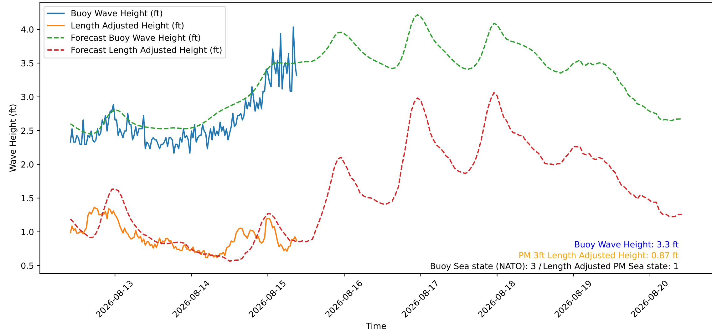
Wave Heights over Time for Red Beach at 2026-08-15 09:50:47
