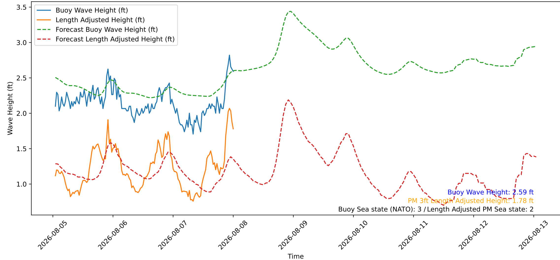
Wave Heights over Time for Green Beach at 2026-08-08 01:01:08
