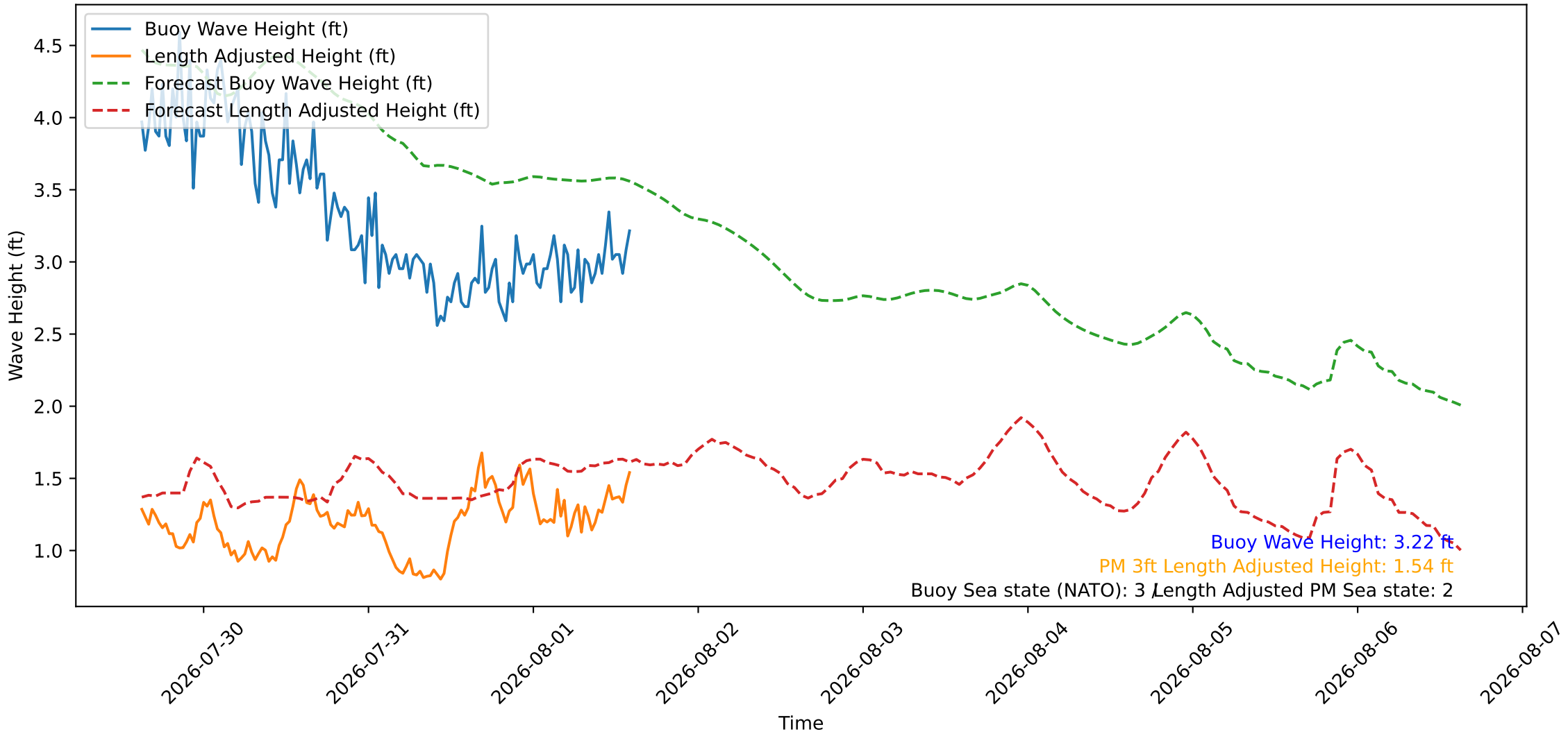
Wave Heights over Time for Red Beach at 2026-08-01 14:40:46
