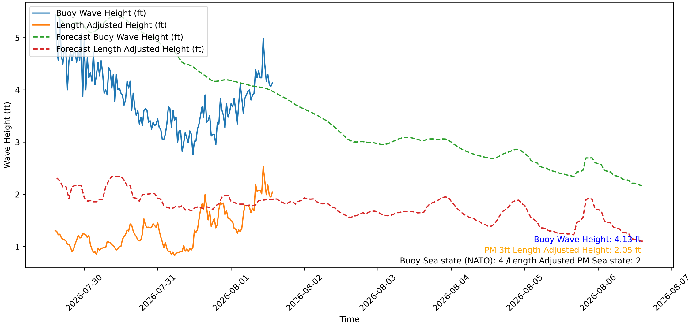
Wave Heights over Time for Green Beach at 2026-08-01 14:41:08
