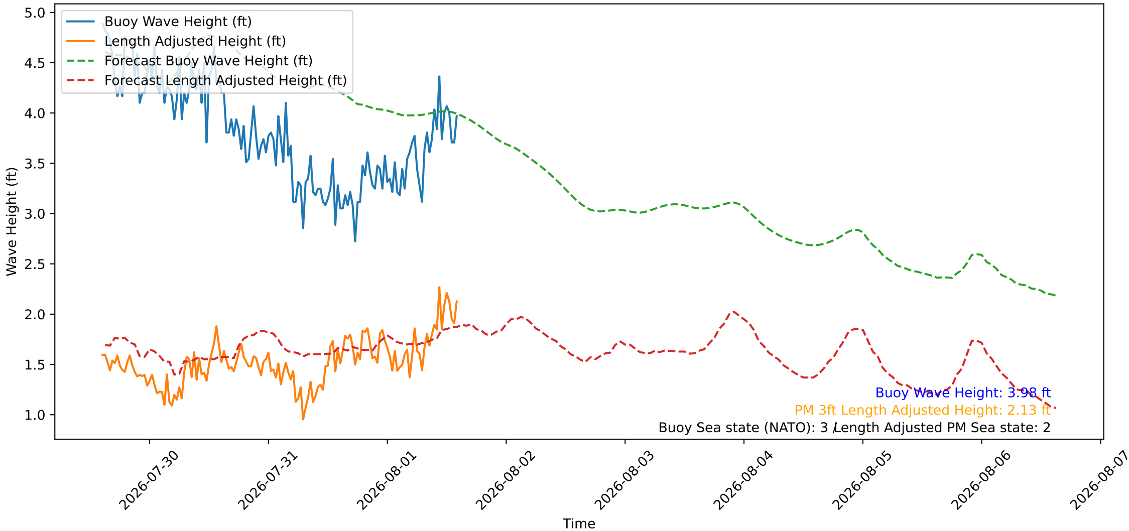
Wave Heights over Time for Oceanside Harbor at 2026-08-01 14:40:26
