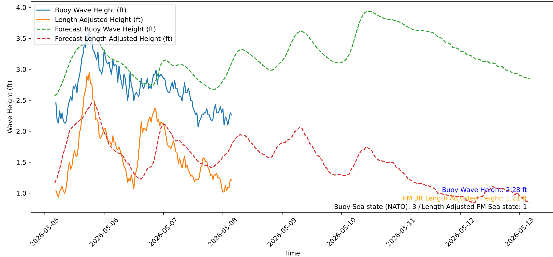
Wave Heights over Time for Green Beach at 2026-05-08 04:21:14
