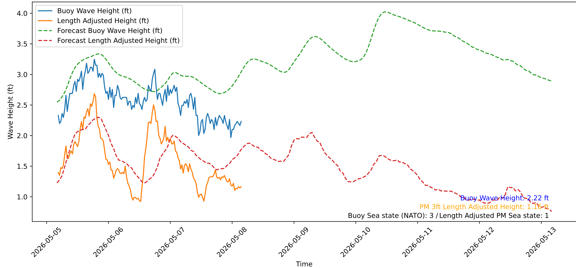
Wave Heights over Time for Oceanside Harbor at 2026-05-08 04:20:31
