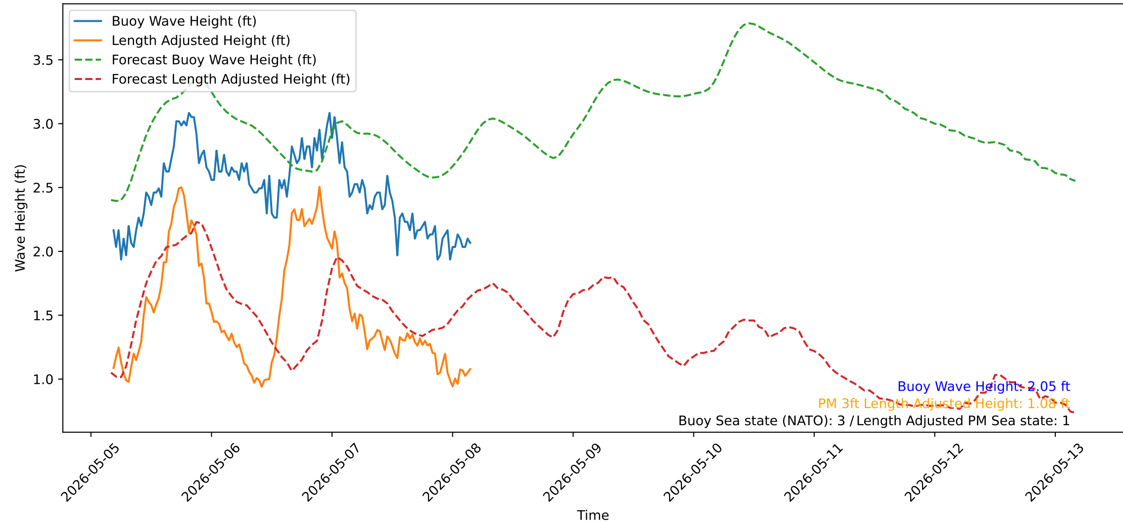
Wave Heights over Time for Red Beach at 2026-05-08 04:20:52
