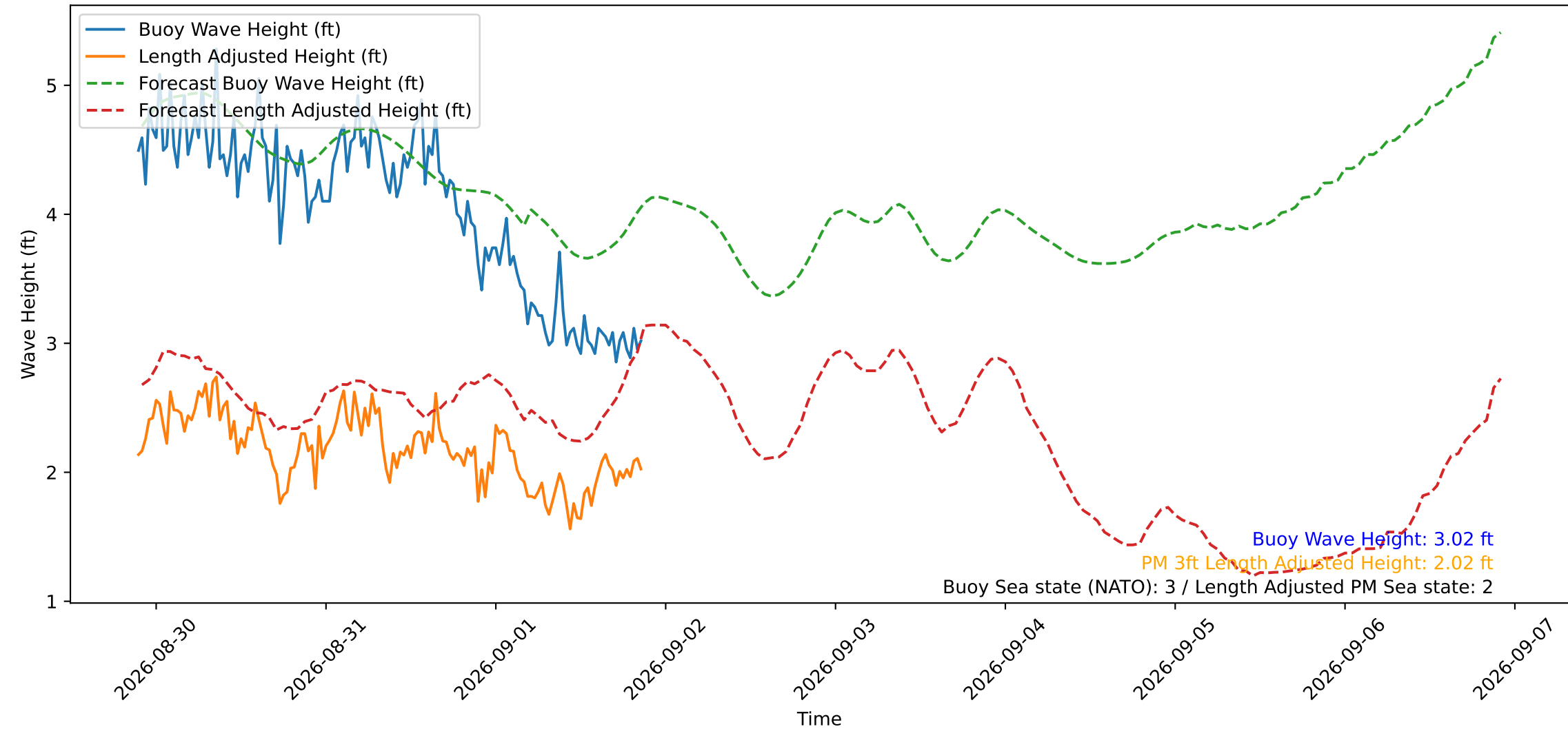
Wave Heights over Time for Oceanside Harbor at 2026-09-01 21:30:30
