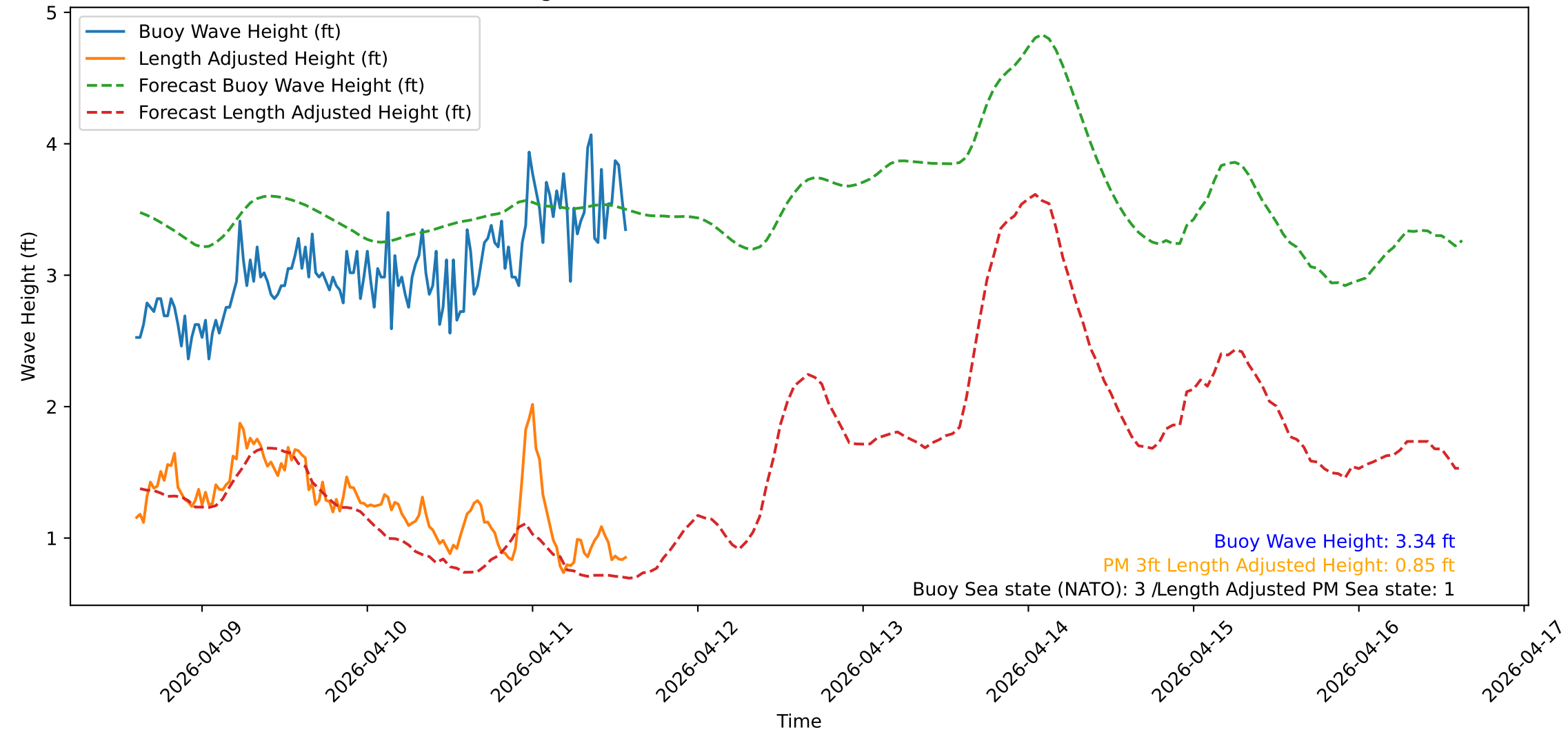
Wave Heights over Time for Green Beach at 2026-04-11 14:31:12
