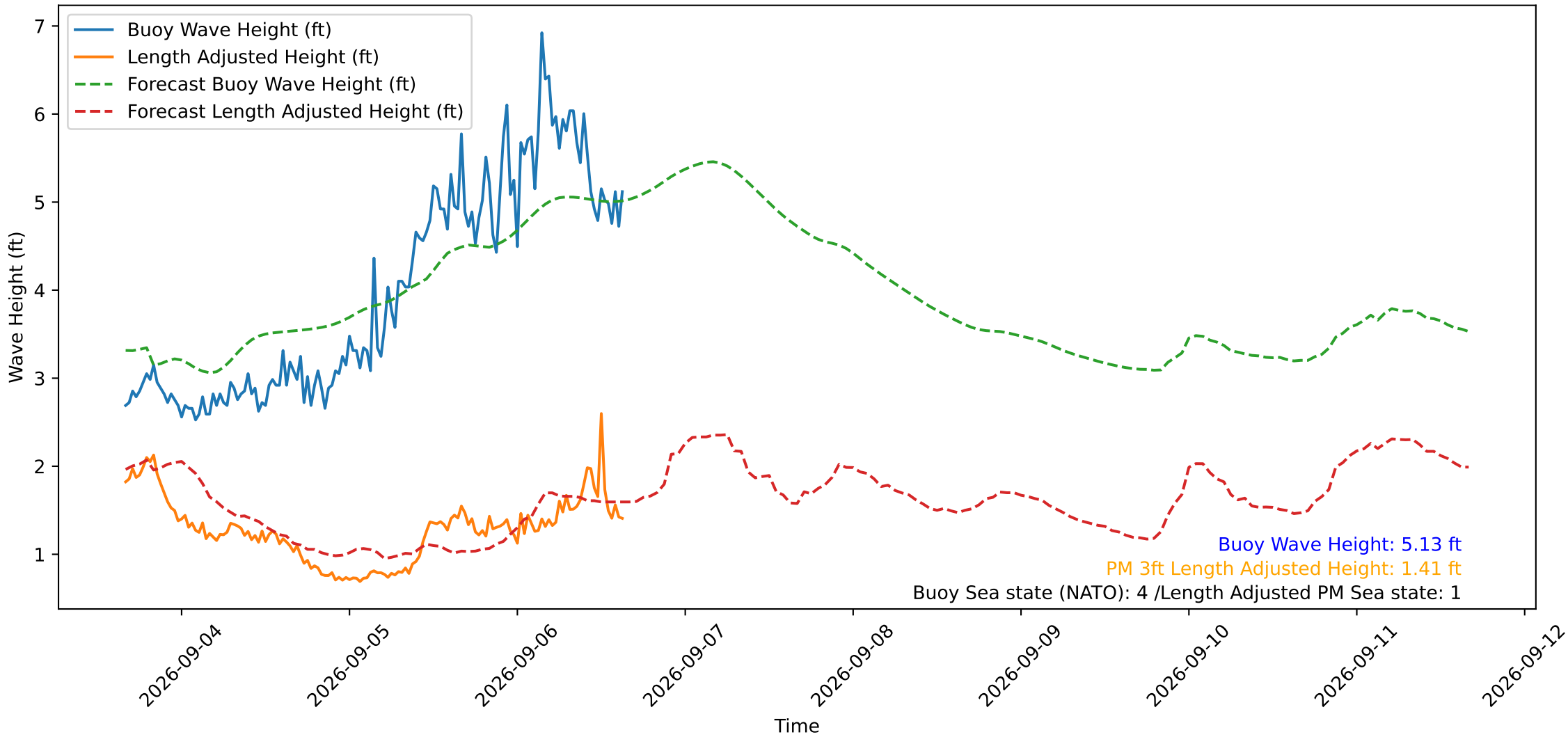
Wave Heights over Time for Red Beach at 2026-09-06 15:50:50
