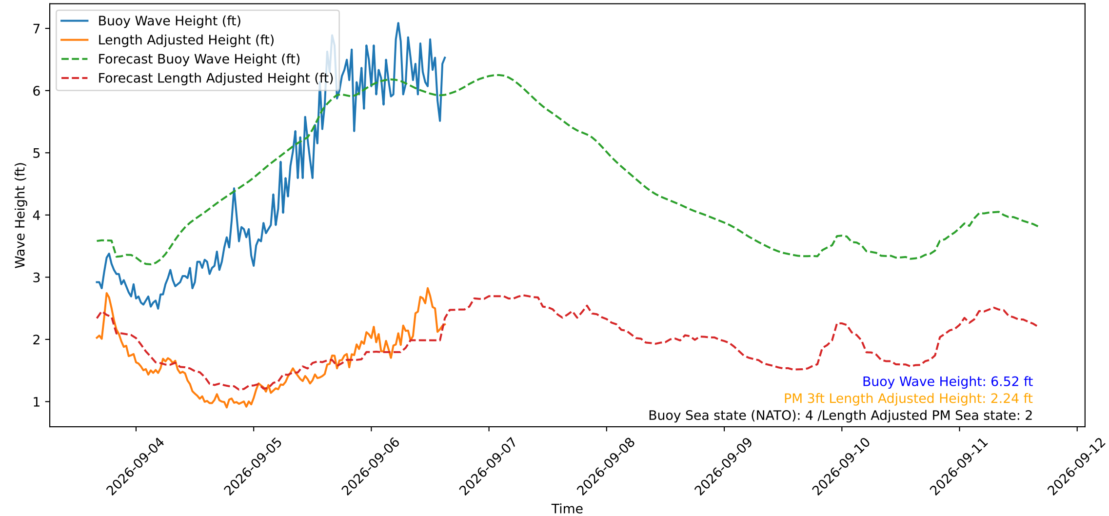
Wave Heights over Time for Green Beach at 2026-09-06 15:51:15
