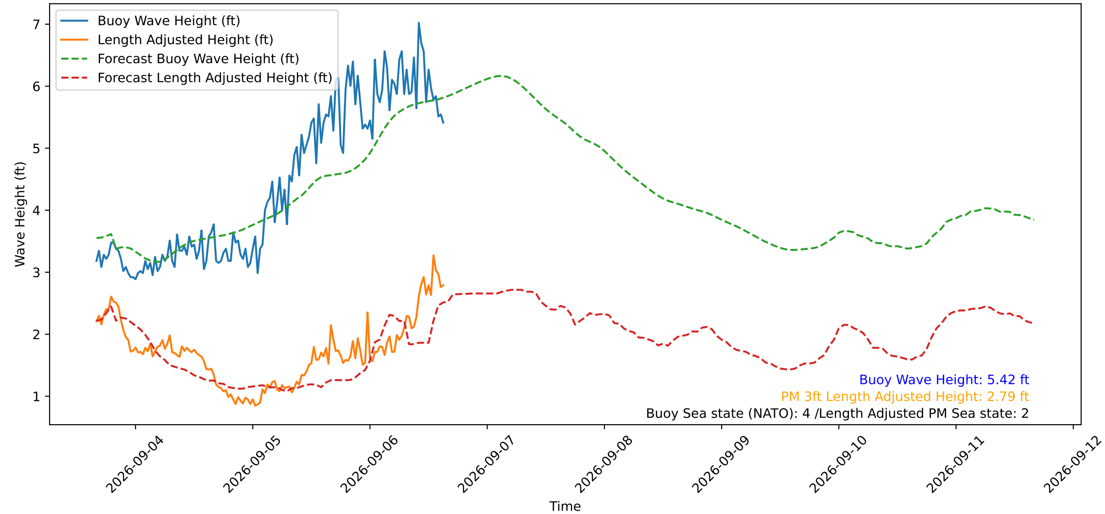
Wave Heights over Time for Oceanside Harbor at 2026-09-06 15:50:29
