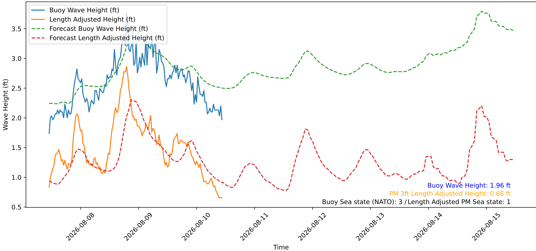
Wave Heights over Time for Green Beach at 2026-08-10 11:11:09
