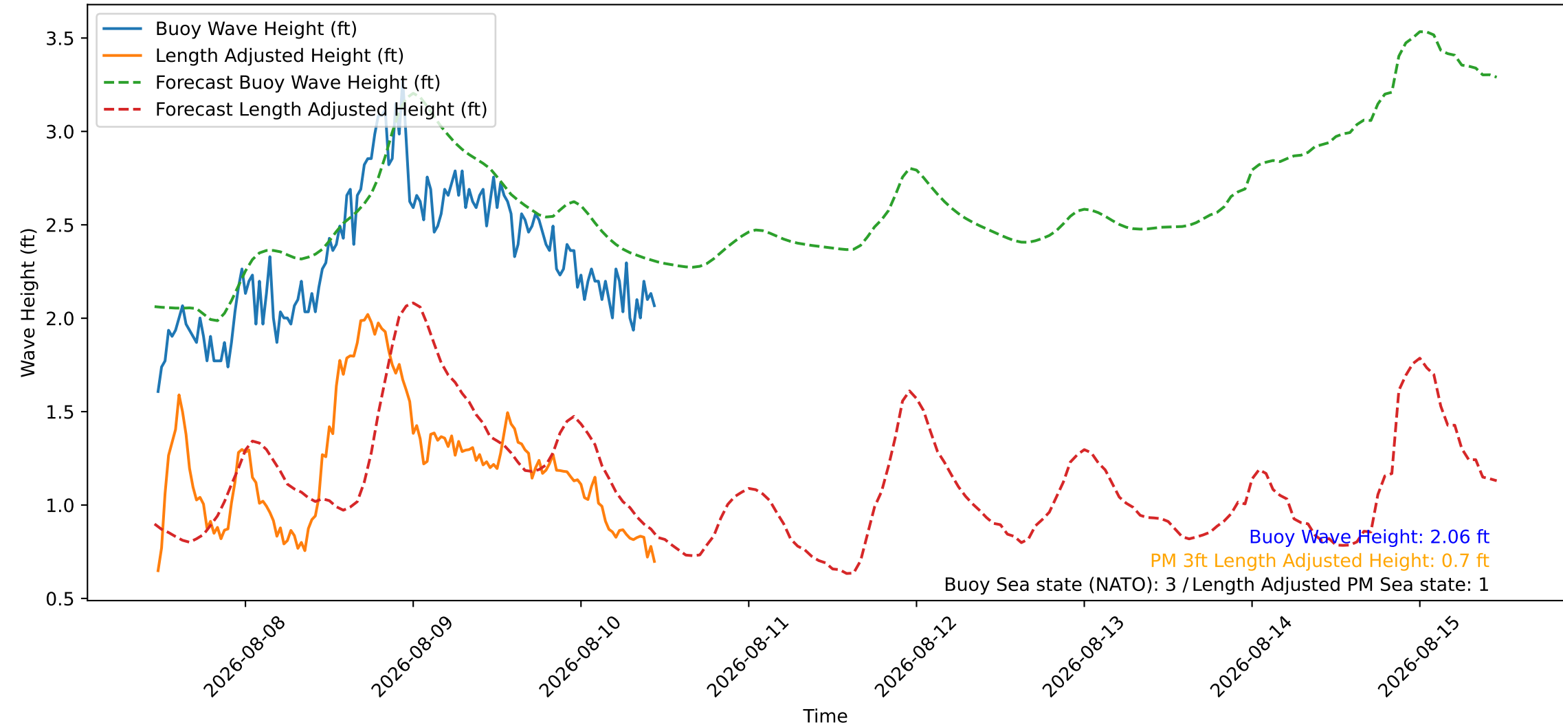
Wave Heights over Time for Red Beach at 2026-08-10 11:10:46
