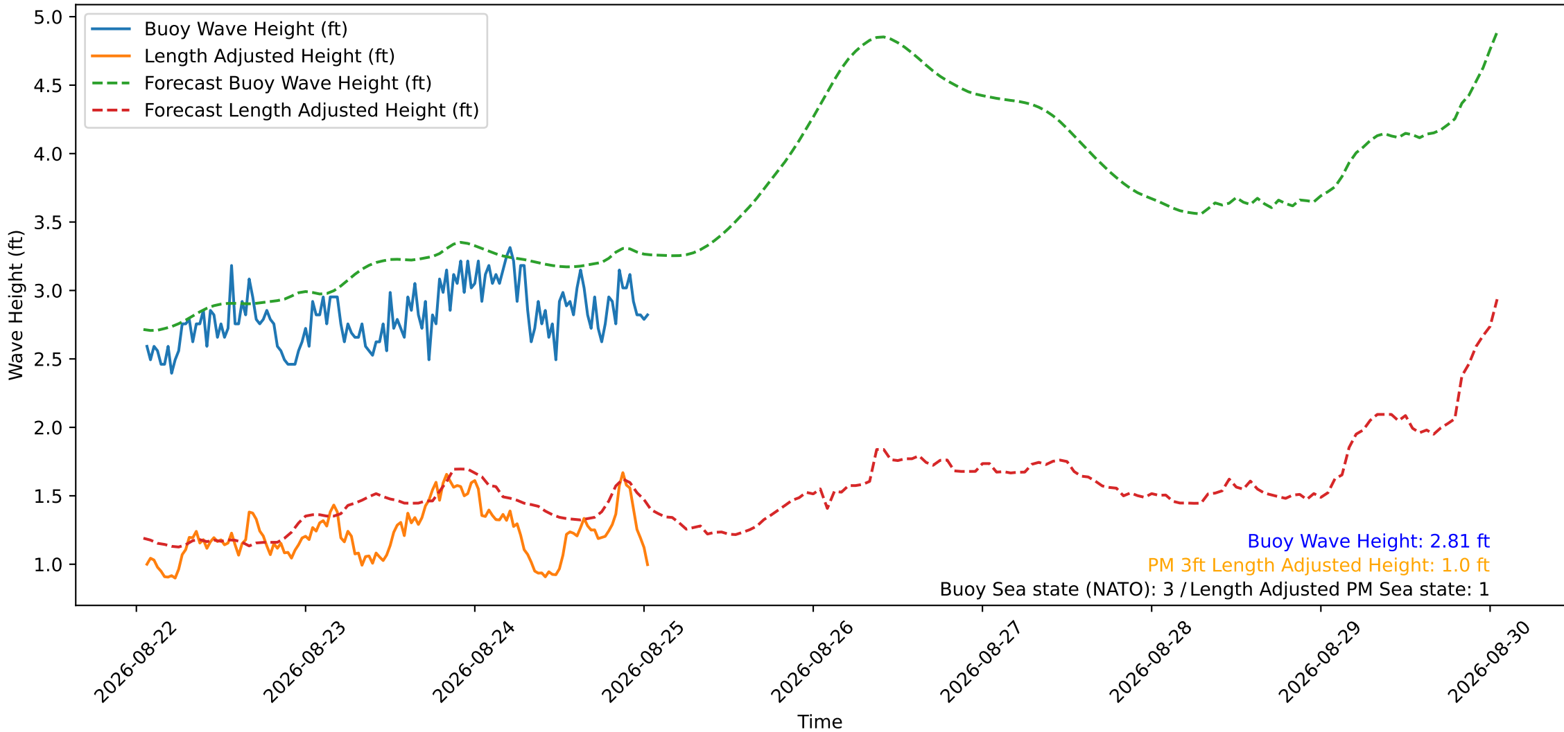
Wave Heights over Time for Green Beach at 2026-08-25 01:21:15
