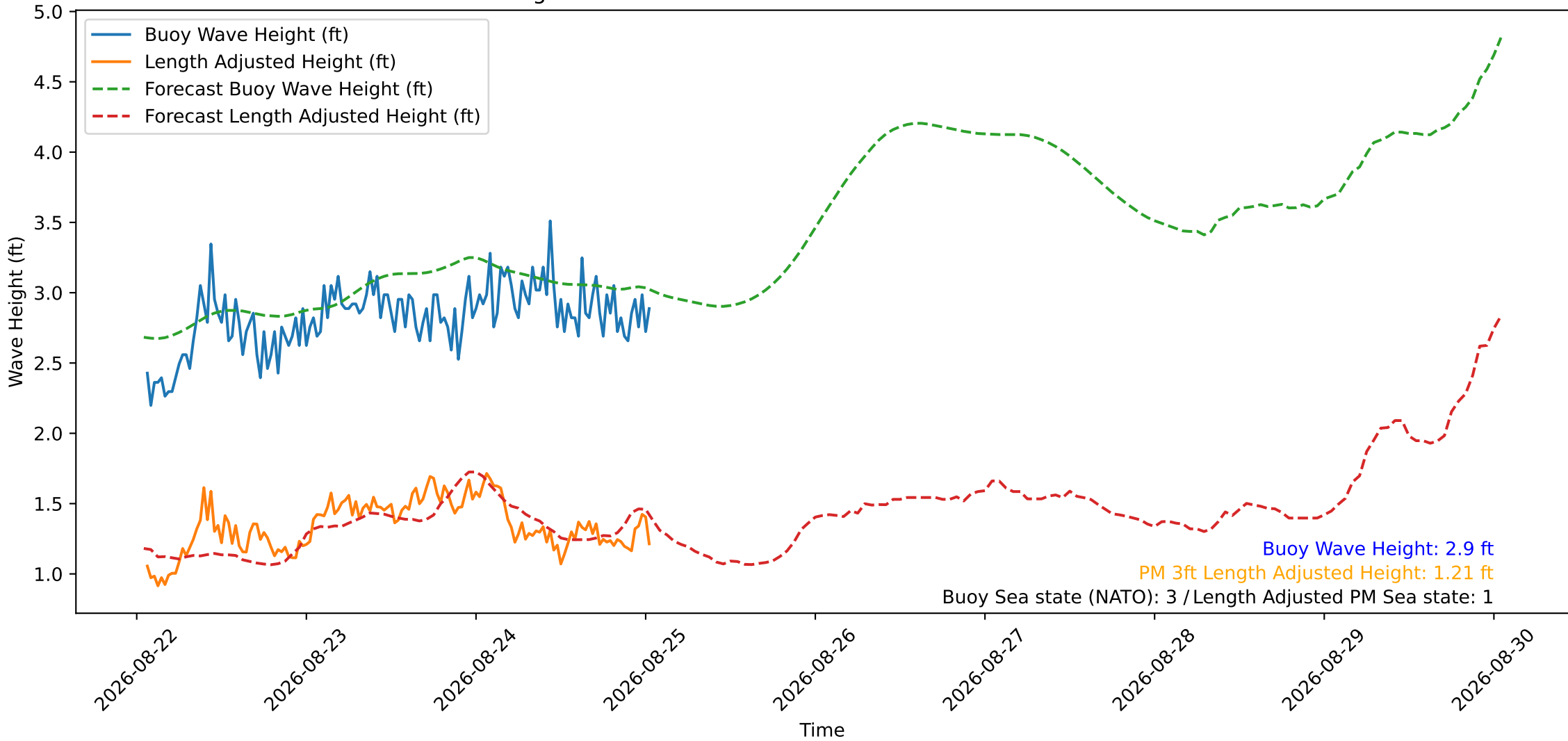
Wave Heights over Time for Oceanside Harbor at 2026-08-25 01:20:30
