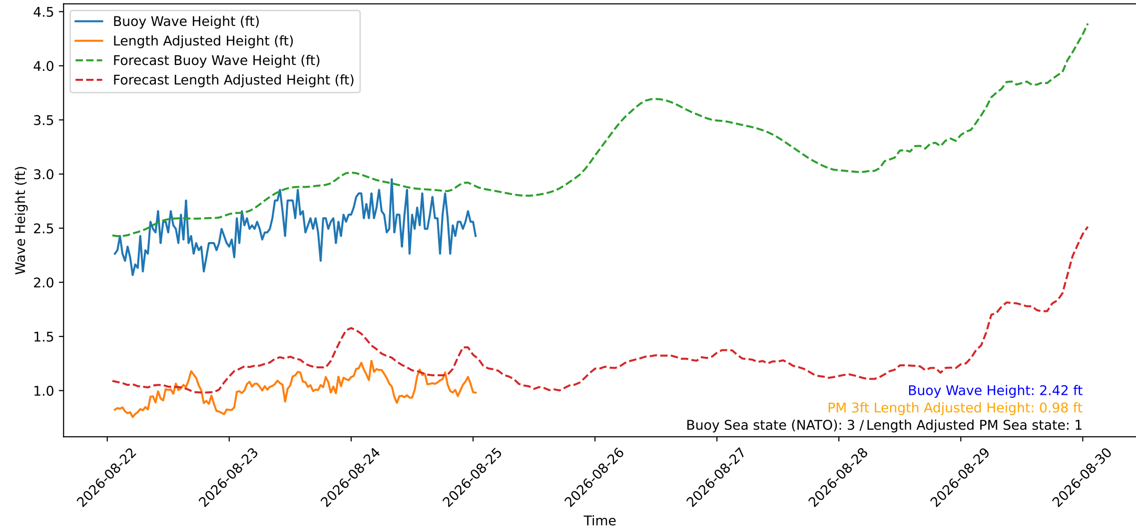
Wave Heights over Time for Red Beach at 2026-08-25 01:20:51
