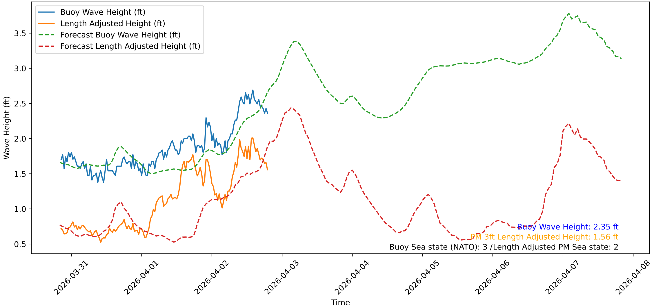
Wave Heights over Time for Red Beach at 2026-04-02 20:10:47
