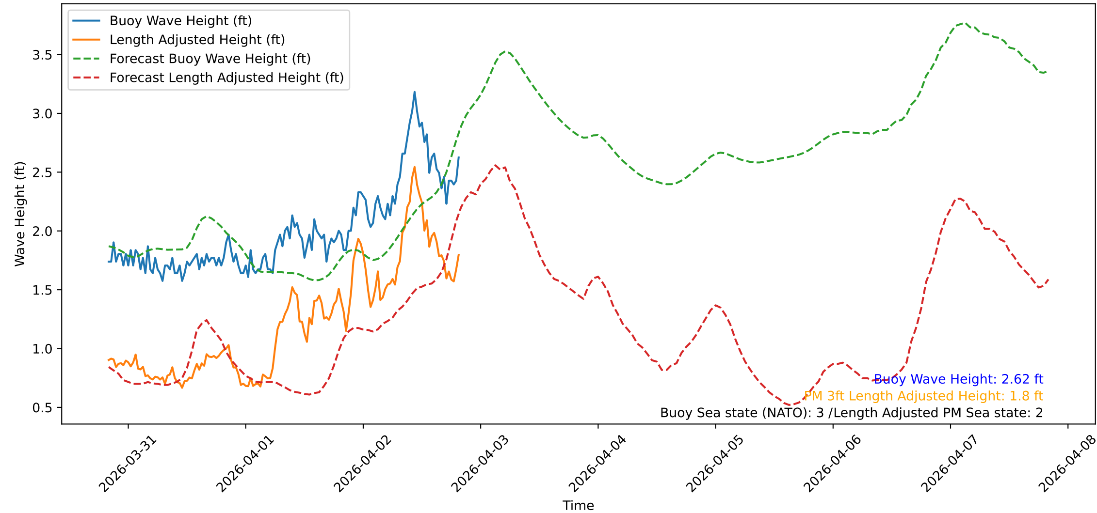
Wave Heights over Time for Oceanside Harbor at 2026-04-02 20:10:31
