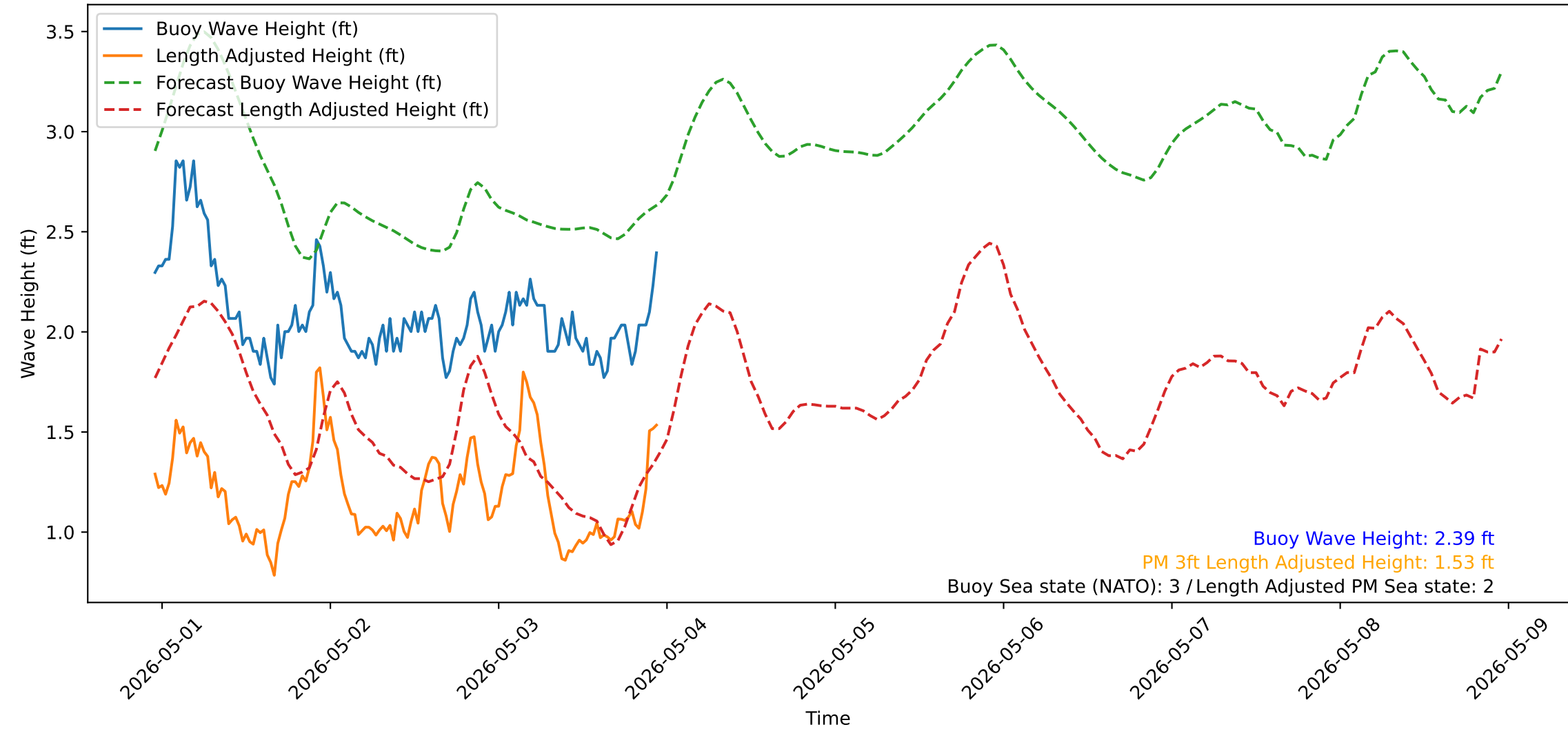
Wave Heights over Time for Green Beach at 2026-05-03 23:11:13
