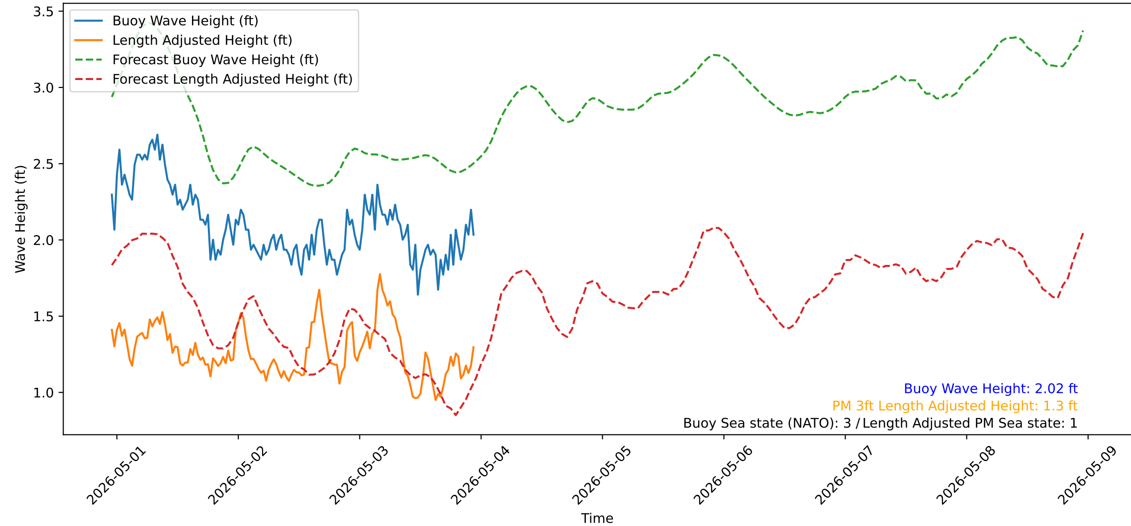
Wave Heights over Time for Oceanside Harbor at 2026-05-03 23:10:31
