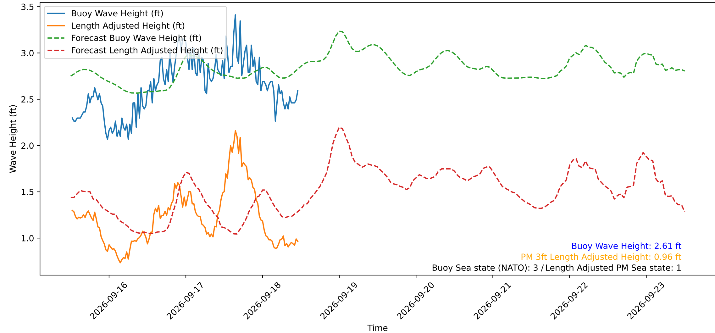
Wave Heights over Time for Red Beach at 2026-09-18 12:00:49
