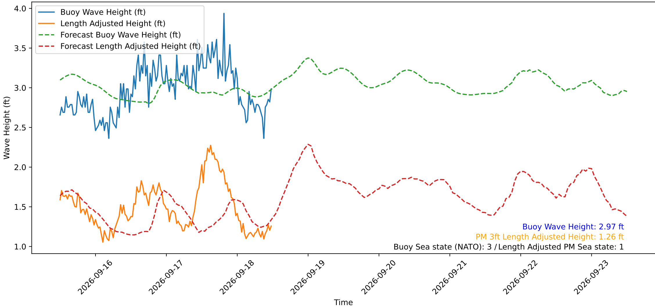
Wave Heights over Time for Oceanside Harbor at 2026-09-18 12:00:30
