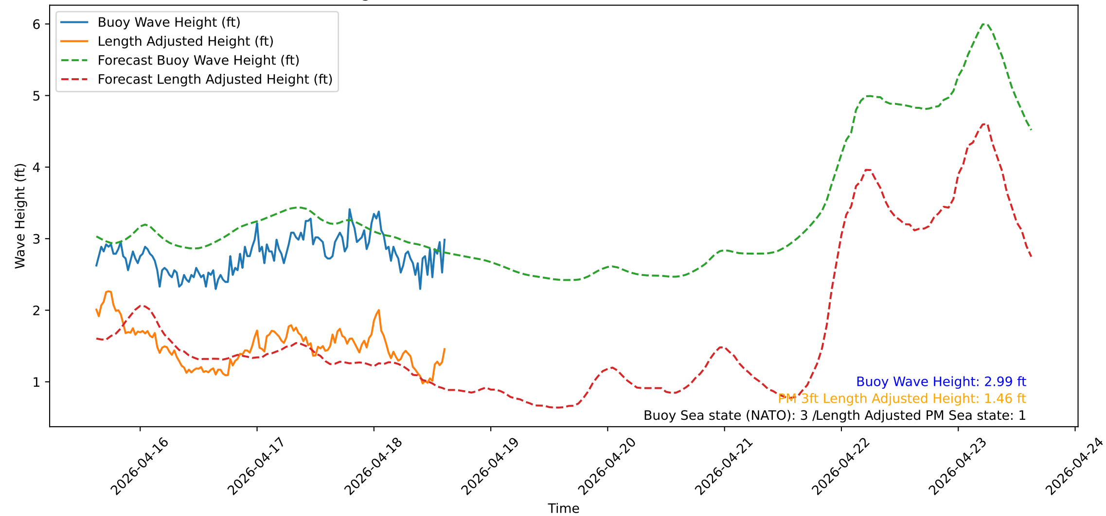
Wave Heights over Time for Oceanside Harbor at 2026-04-18 15:10:31
