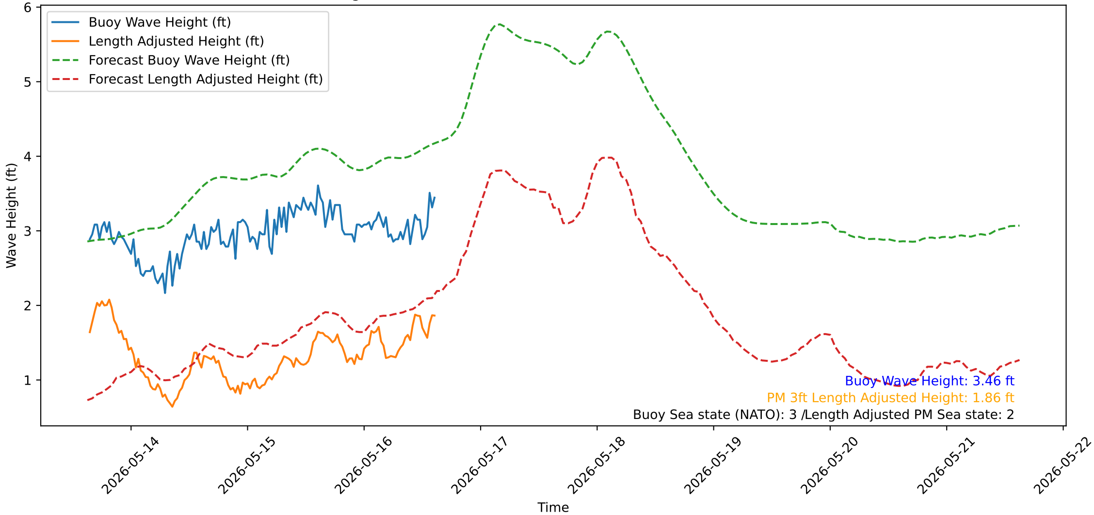
Wave Heights over Time for Oceanside Harbor at 2026-05-16 15:20:31
