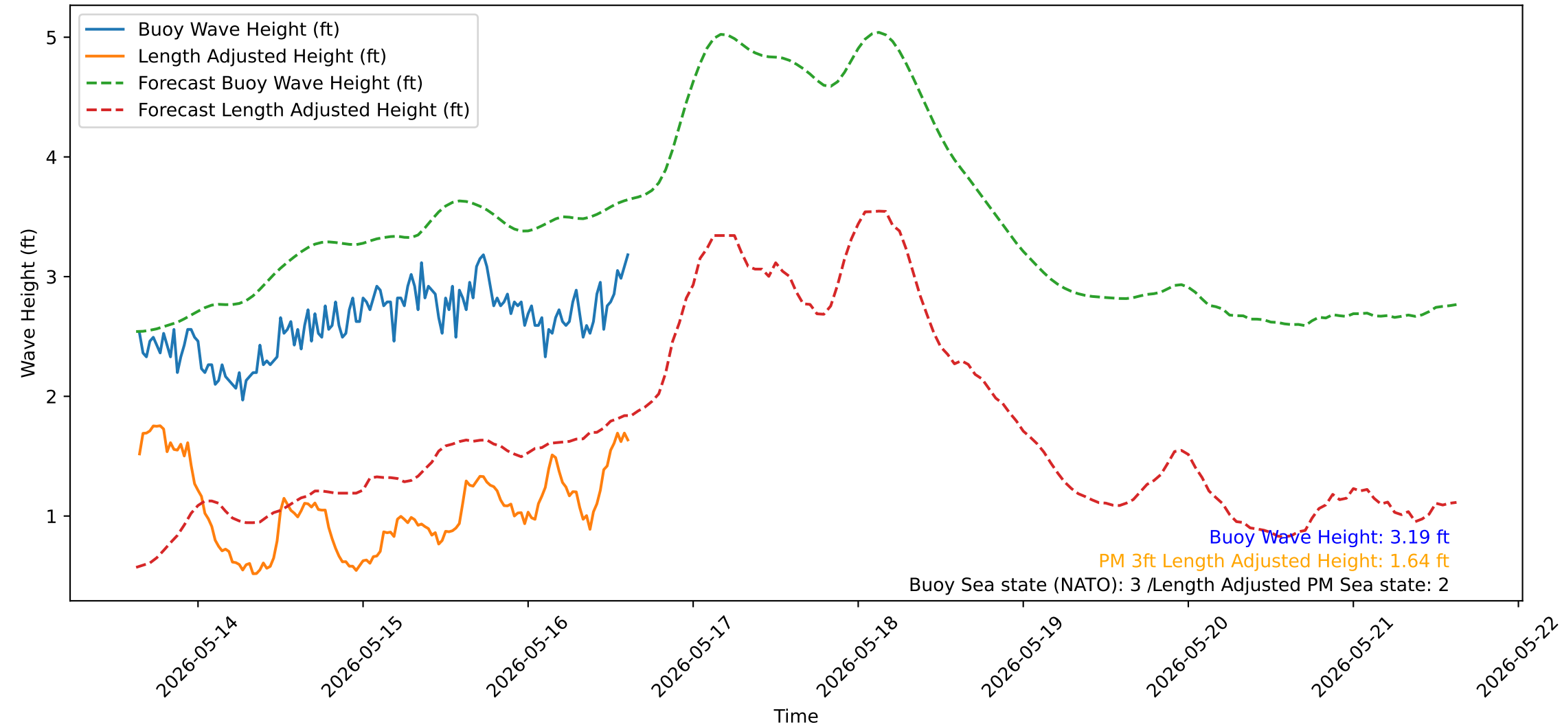
Wave Heights over Time for Red Beach at 2026-05-16 15:20:53
