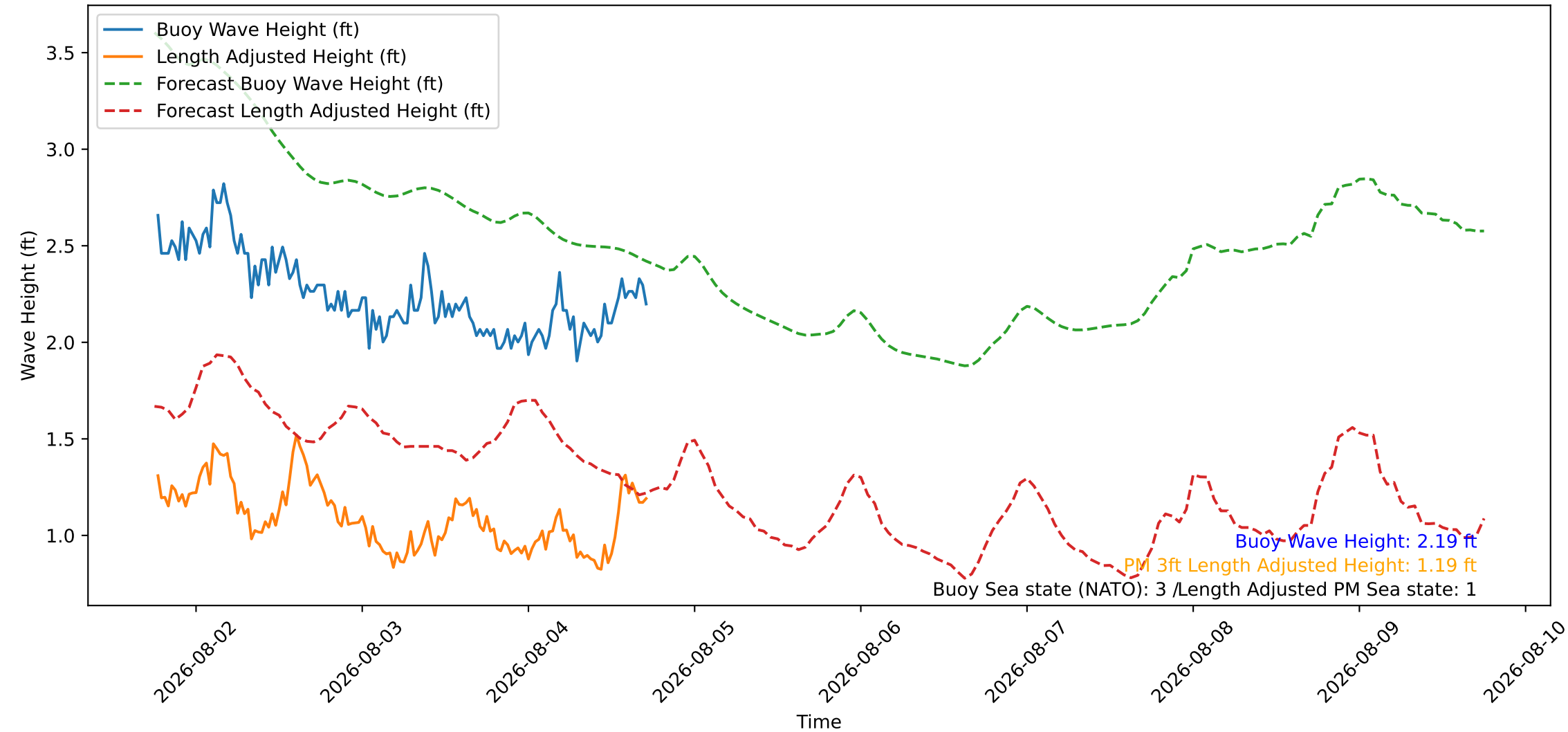
Wave Heights over Time for Red Beach at 2026-08-04 18:00:46
