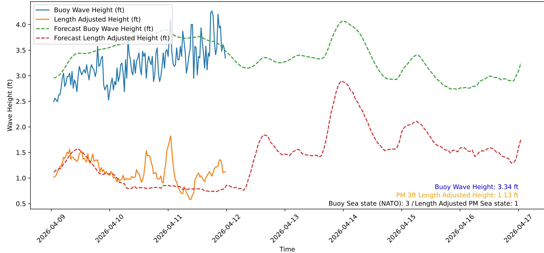
Wave Heights over Time for Red Beach at 2026-04-12 00:50:53
