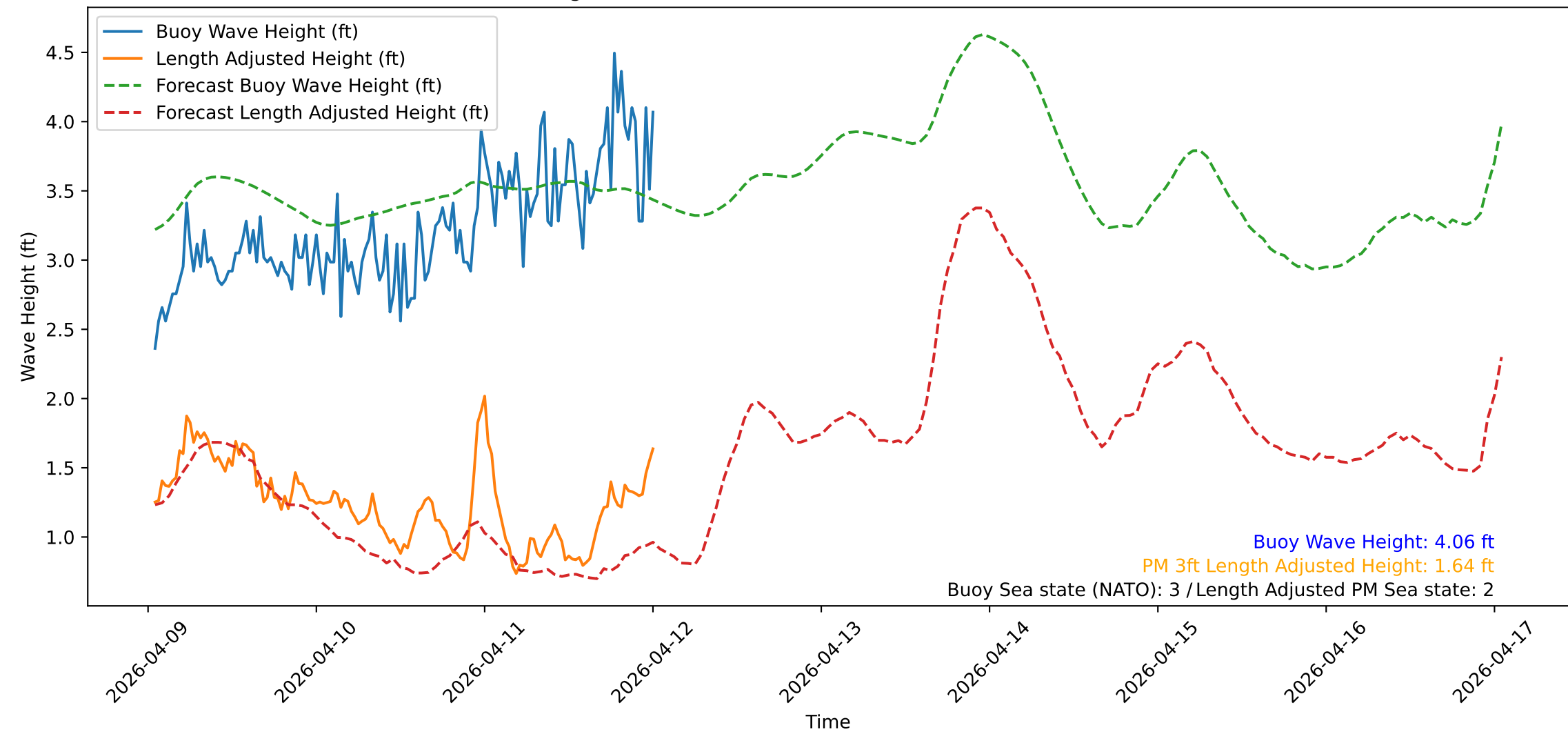
Wave Heights over Time for Green Beach at 2026-04-12 00:51:16
