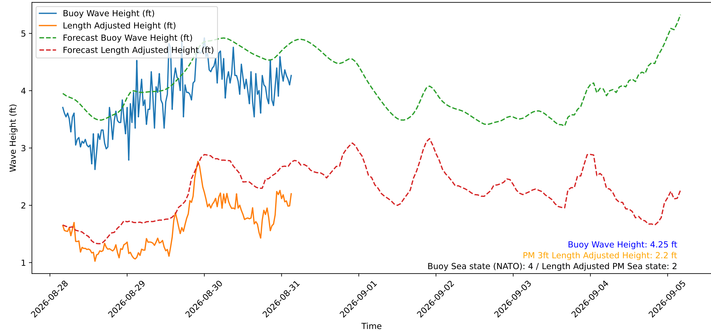
Wave Heights over Time for Green Beach at 2026-08-31 03:41:13
