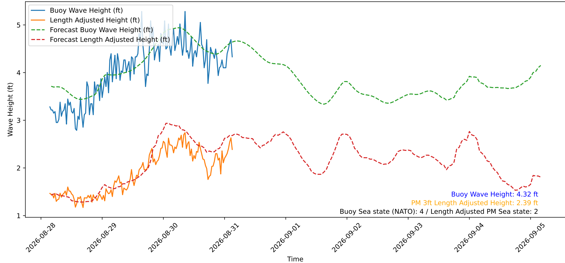
Wave Heights over Time for Oceanside Harbor at 2026-08-31 03:40:30
