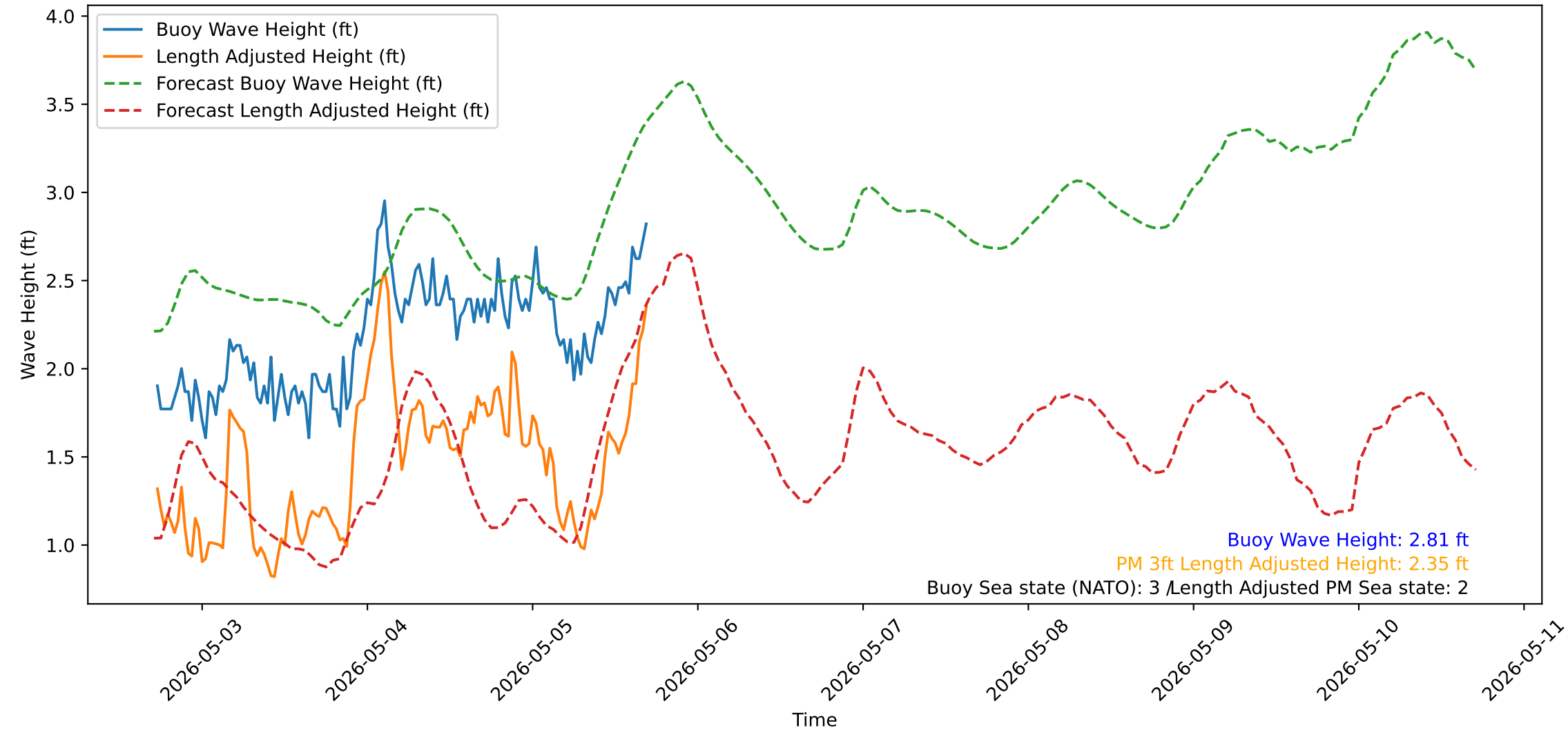
Wave Heights over Time for Red Beach at 2026-05-05 17:20:52
