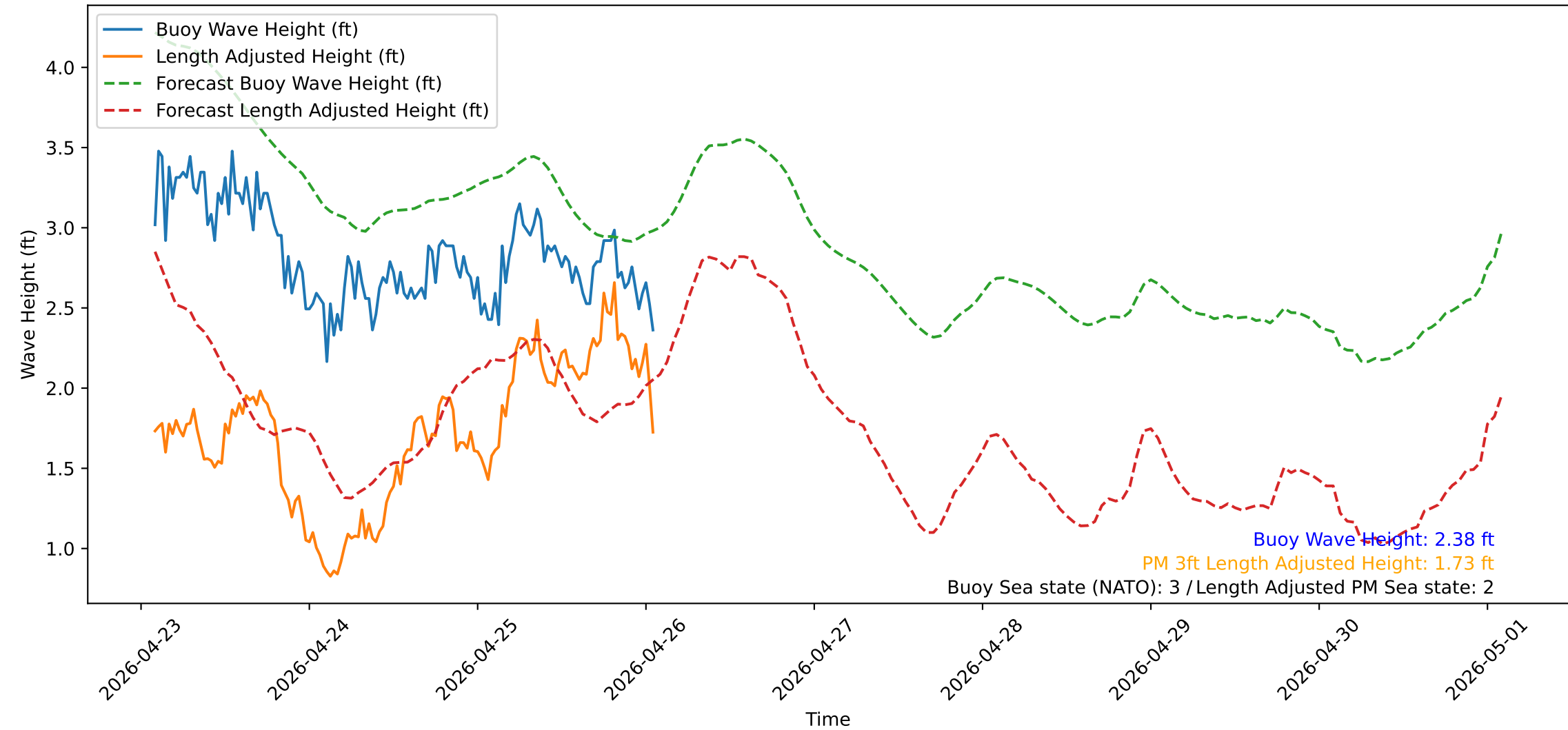
Wave Heights over Time for Red Beach at 2026-04-26 01:40:50
