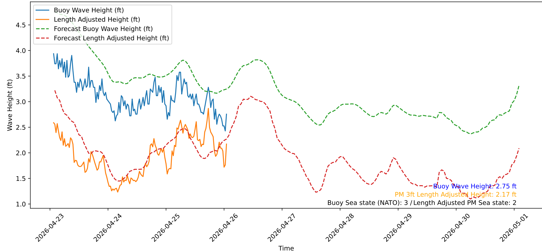
Wave Heights over Time for Green Beach at 2026-04-26 01:41:13
