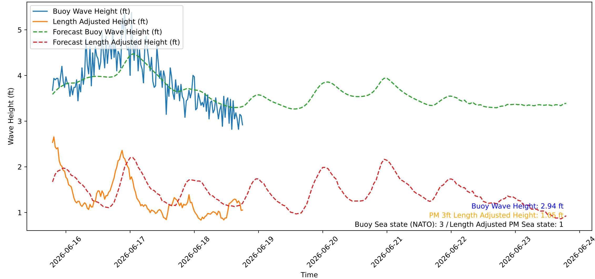
Wave Heights over Time for Red Beach at 2026-06-18 18:50:46
