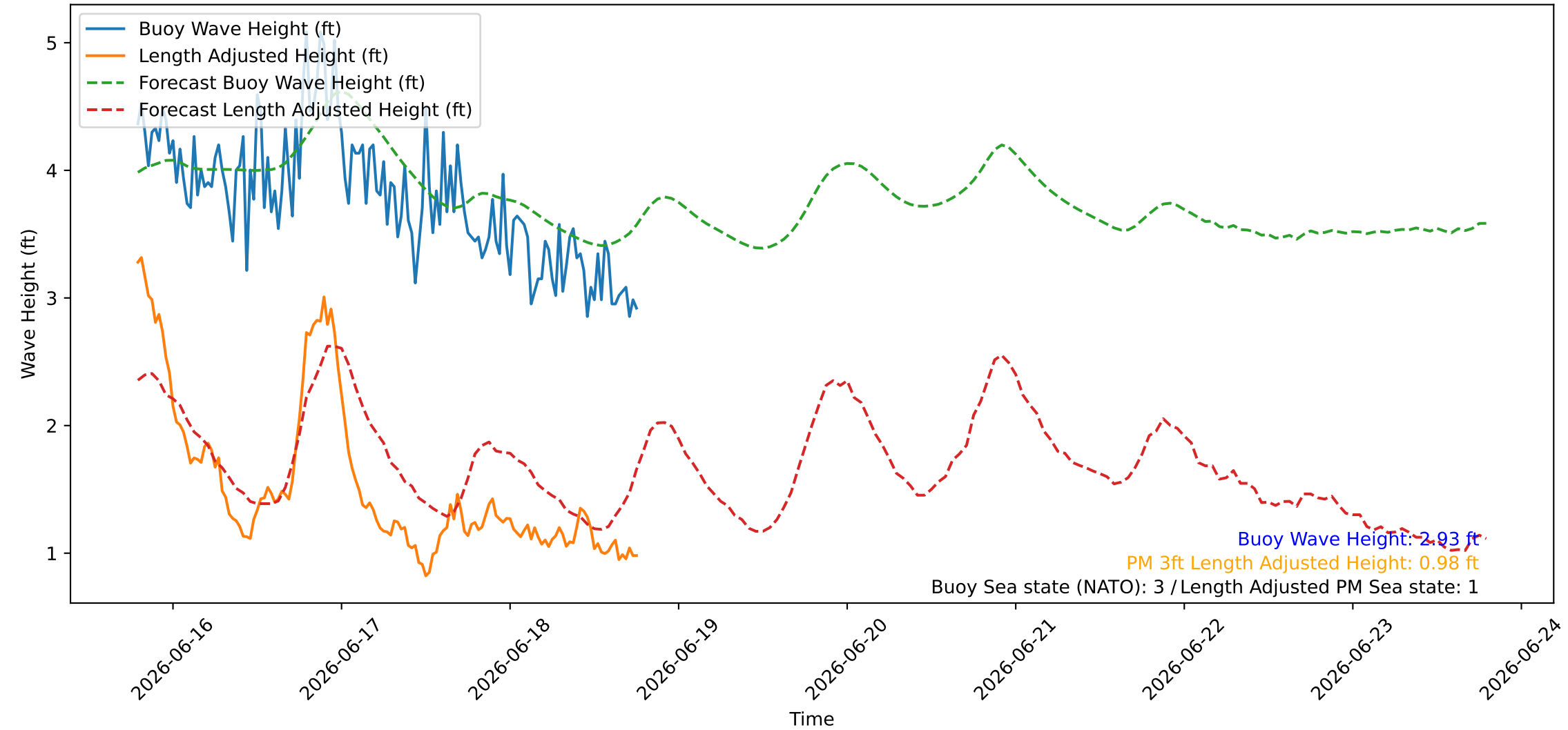
Wave Heights over Time for Green Beach at 2026-06-18 18:51:08
