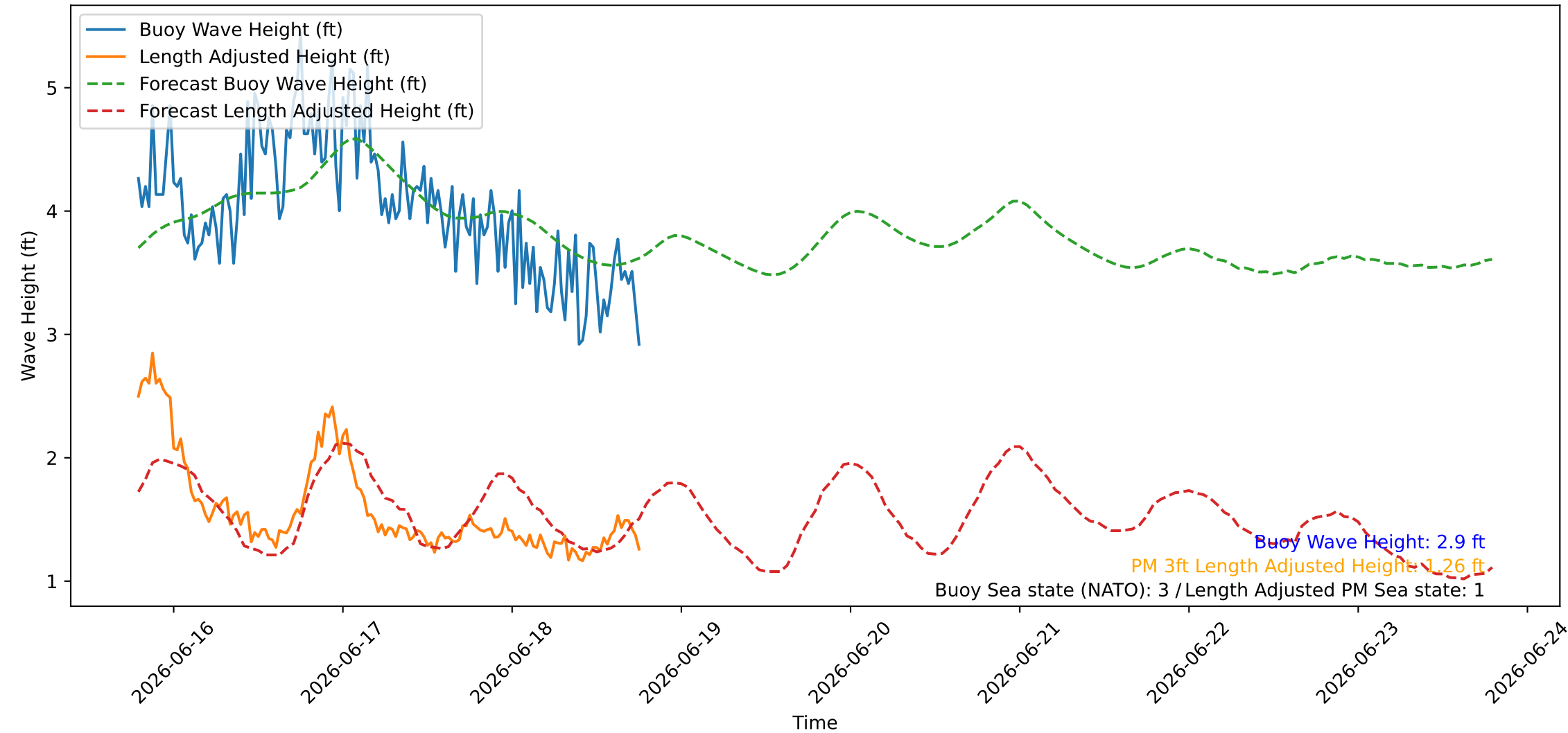
Wave Heights over Time for Oceanside Harbor at 2026-06-18 18:50:26
