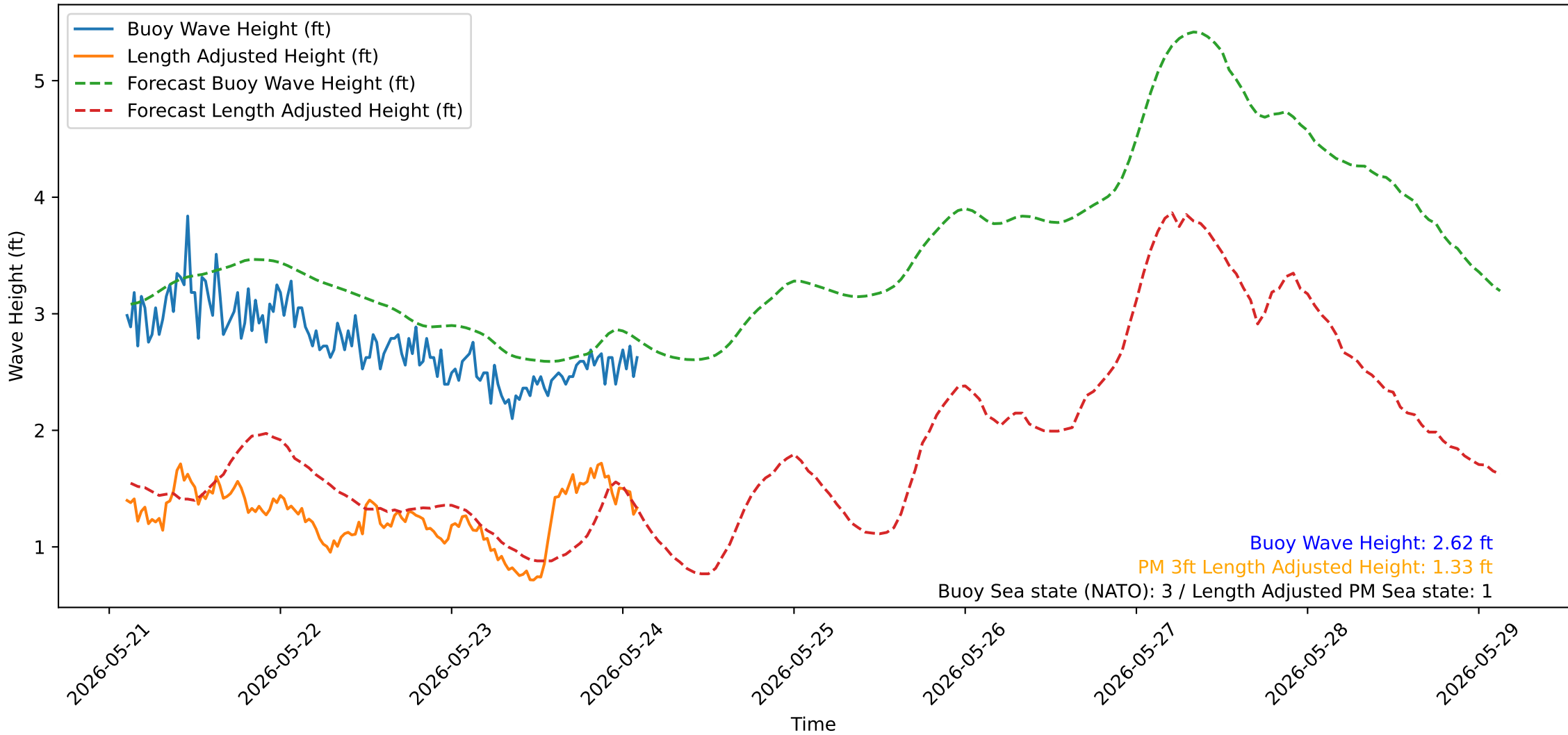
Wave Heights over Time for Oceanside Harbor at 2026-05-24 02:40:32
