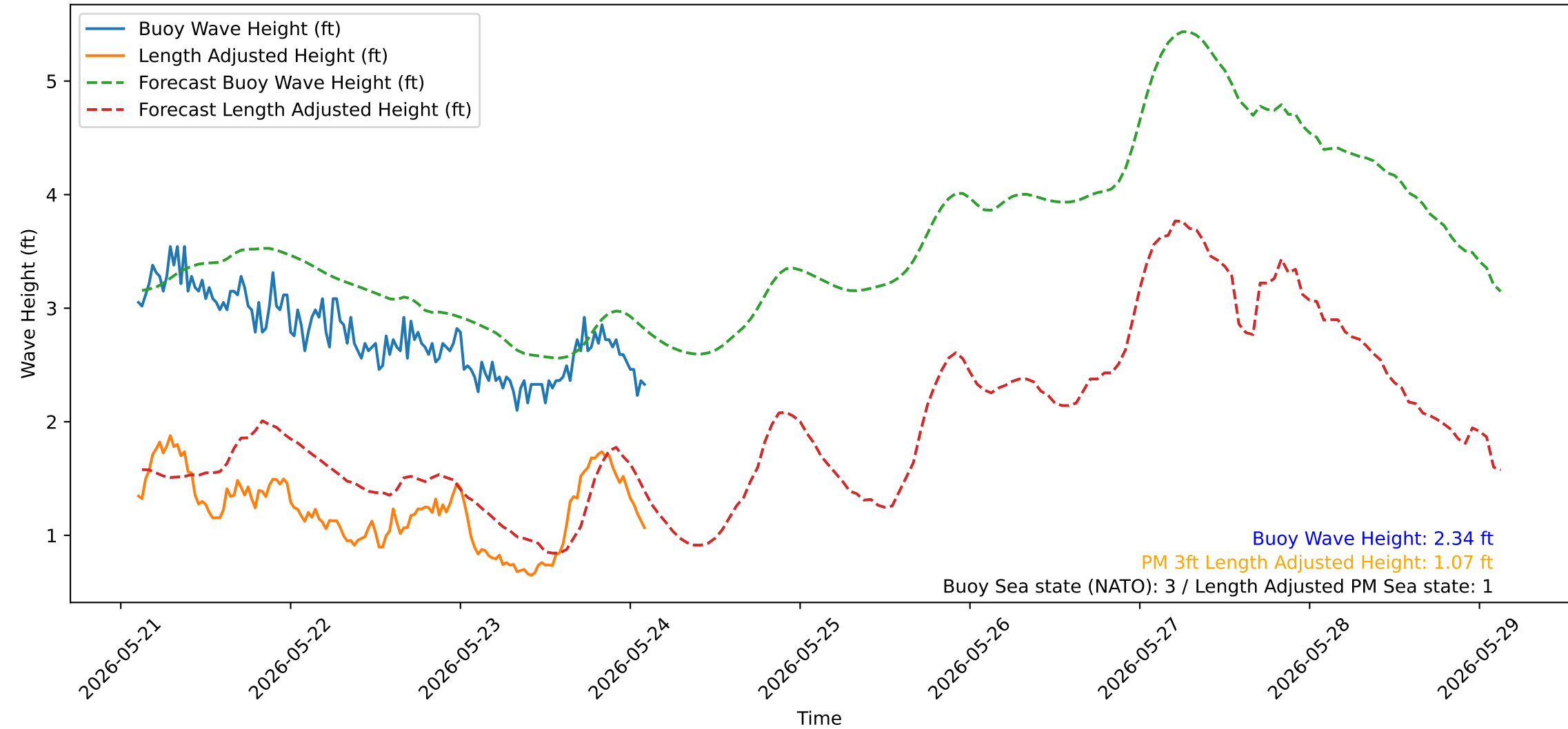
Wave Heights over Time for Green Beach at 2026-05-24 02:41:14
