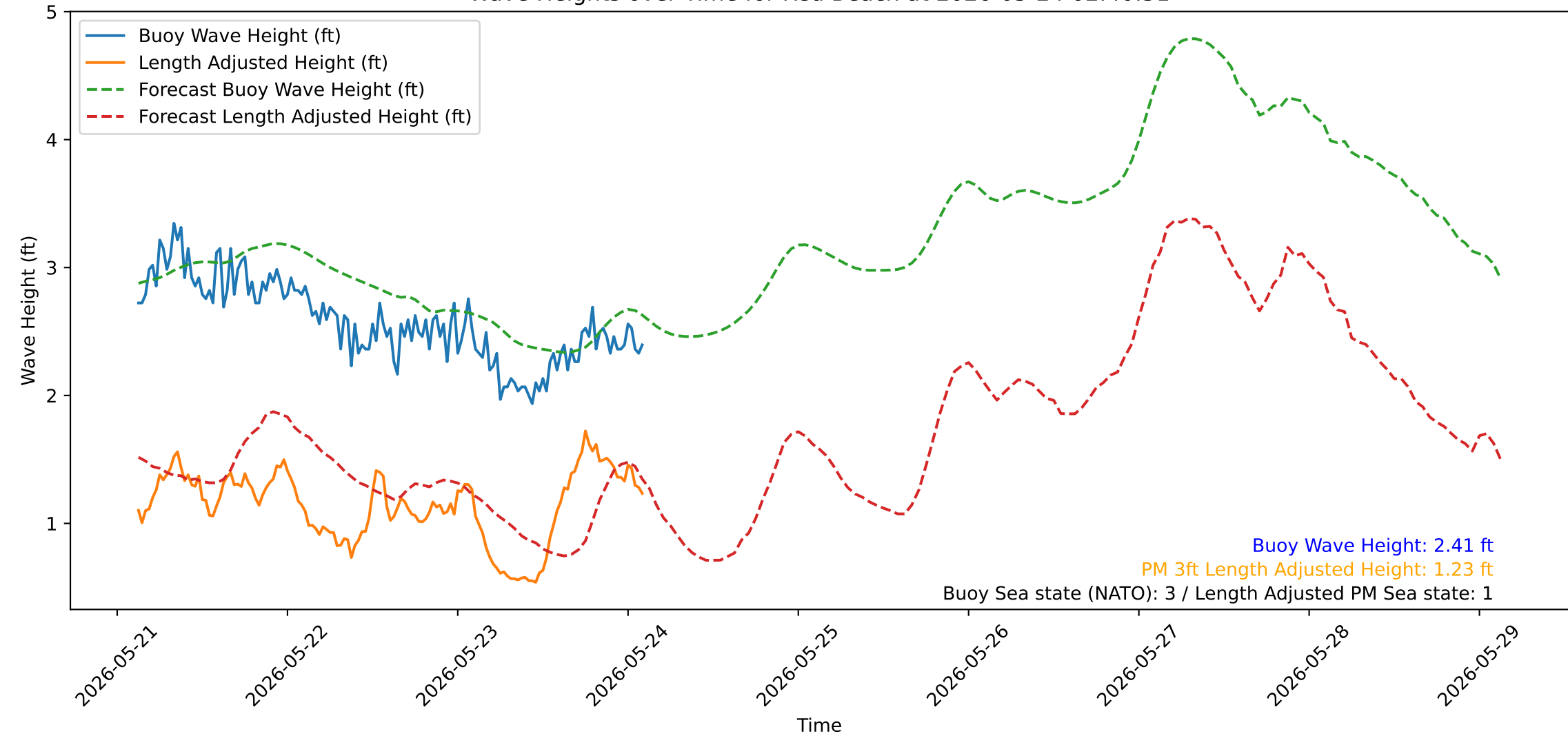
Wave Heights over Time for Red Beach at 2026-05-24 02:40:51
