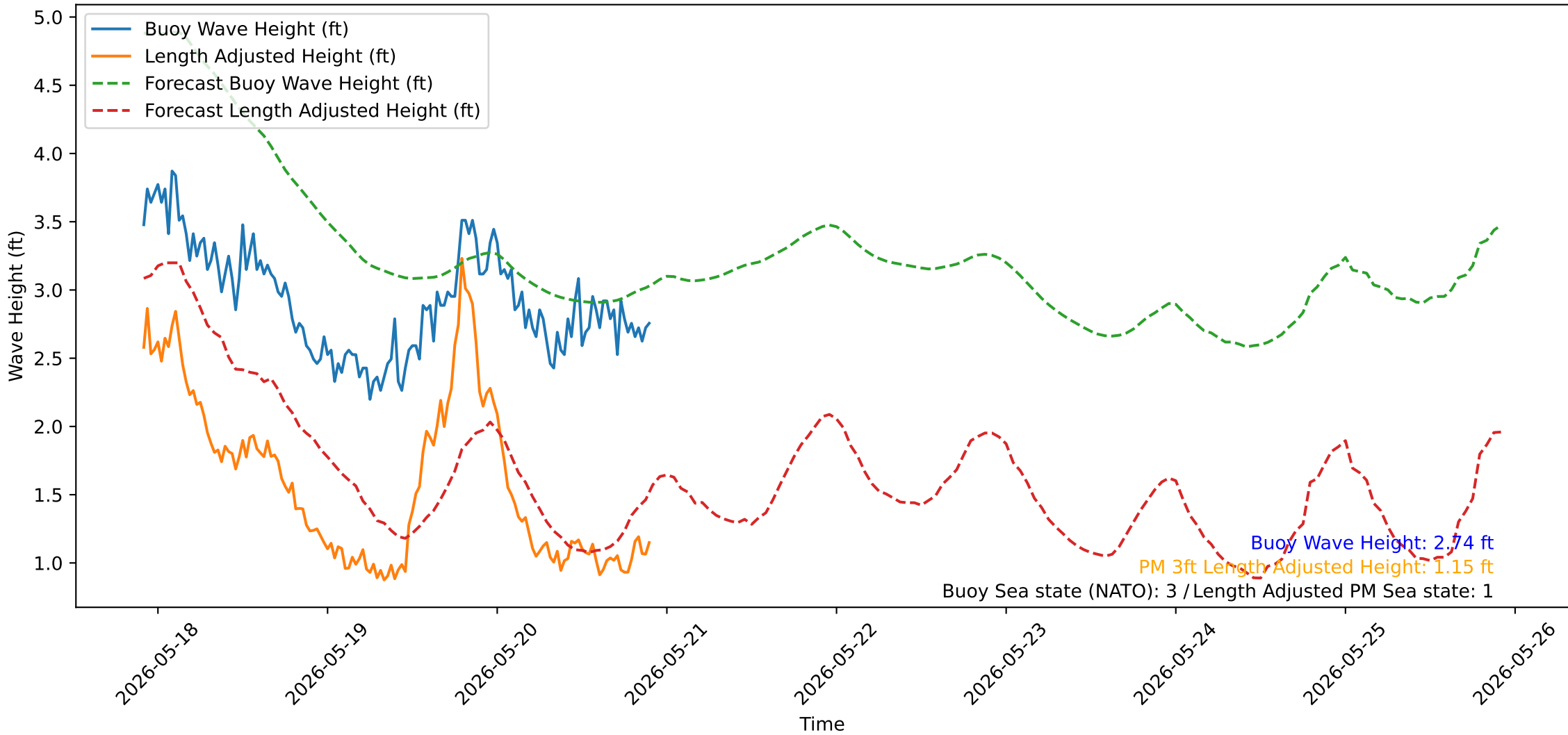
Wave Heights over Time for Oceanside Harbor at 2026-05-20 22:00:32
