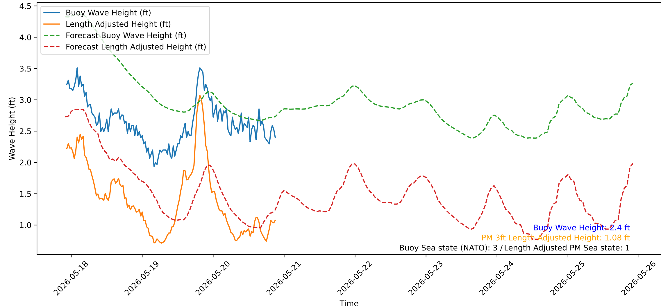
Wave Heights over Time for Red Beach at 2026-05-20 22:00:52
