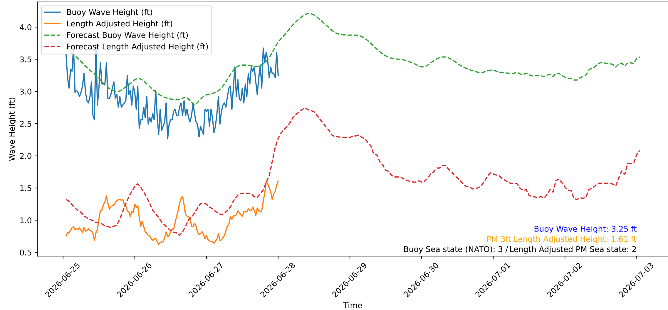
Wave Heights over Time for Red Beach at 2026-06-28 00:50:47
