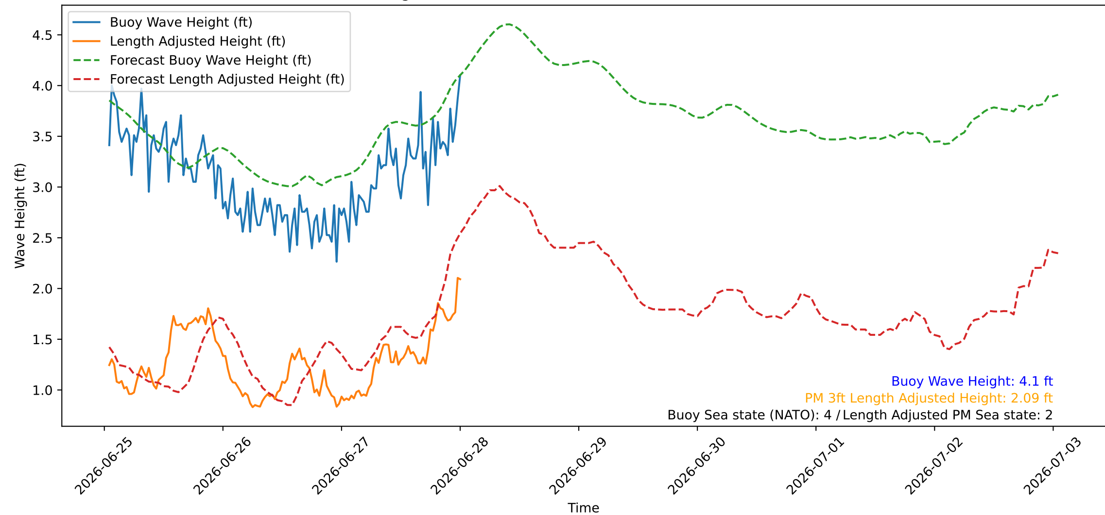
Wave Heights over Time for Green Beach at 2026-06-28 00:51:09
