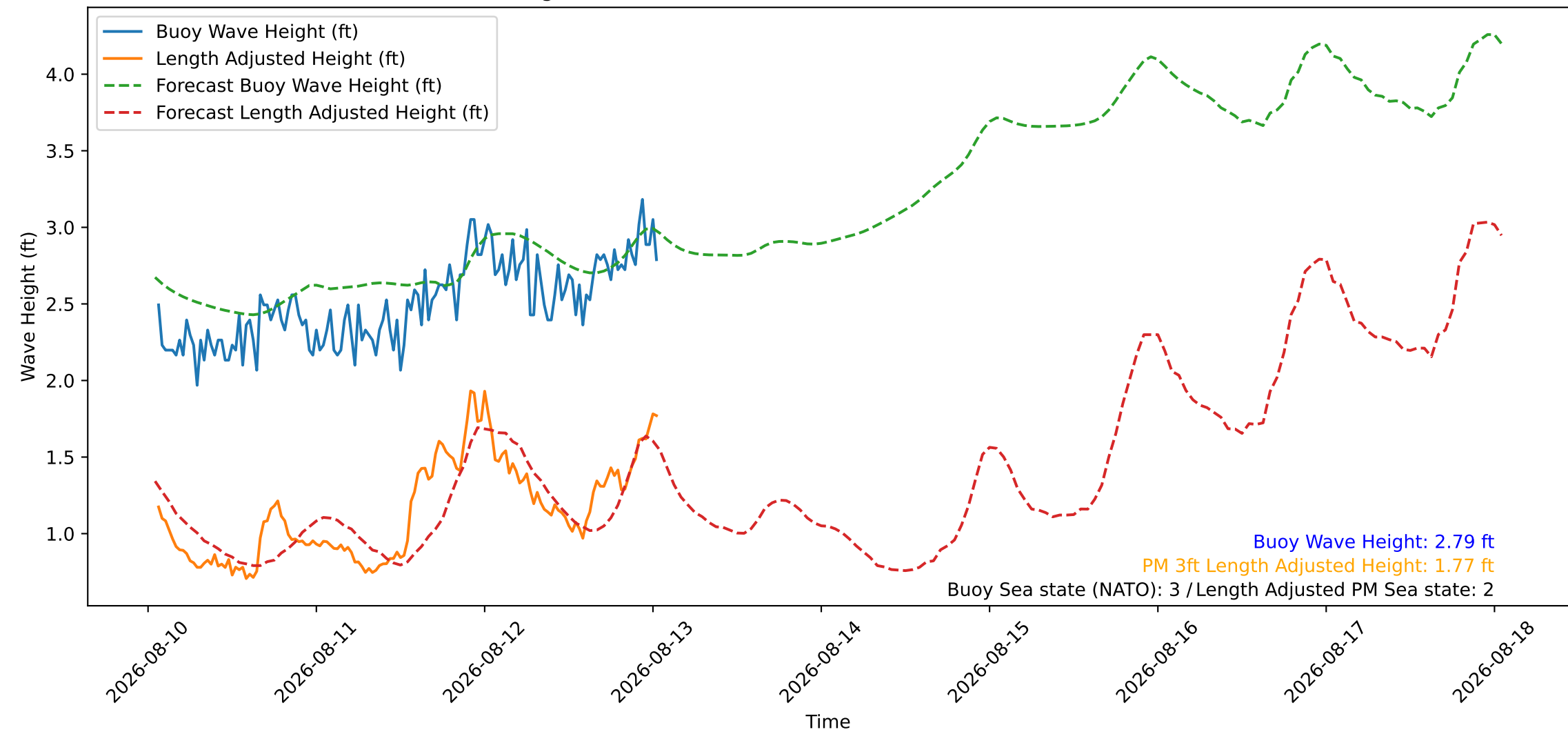
Wave Heights over Time for Oceanside Harbor at 2026-08-13 01:20:26
