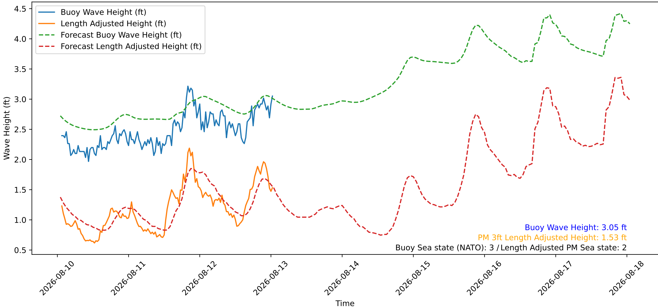
Wave Heights over Time for Green Beach at 2026-08-13 01:21:09
