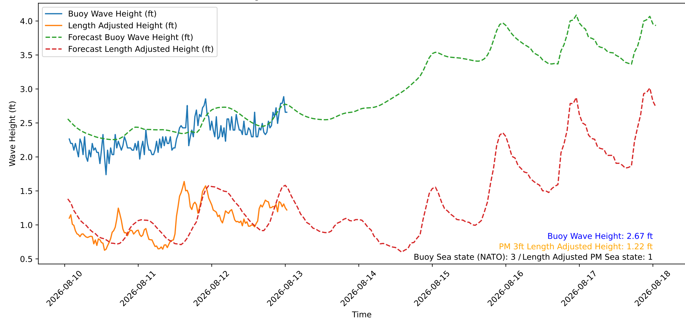
Wave Heights over Time for Red Beach at 2026-08-13 01:20:46
