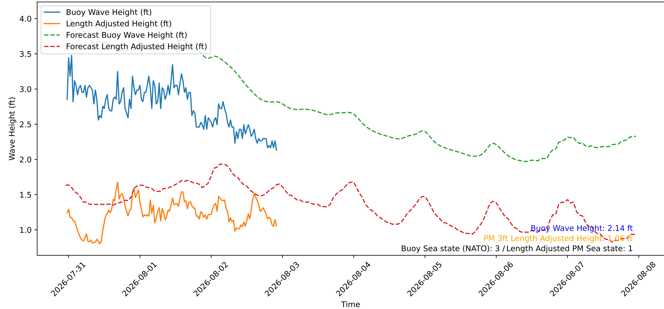
Wave Heights over Time for Red Beach at 2026-08-02 23:20:47
