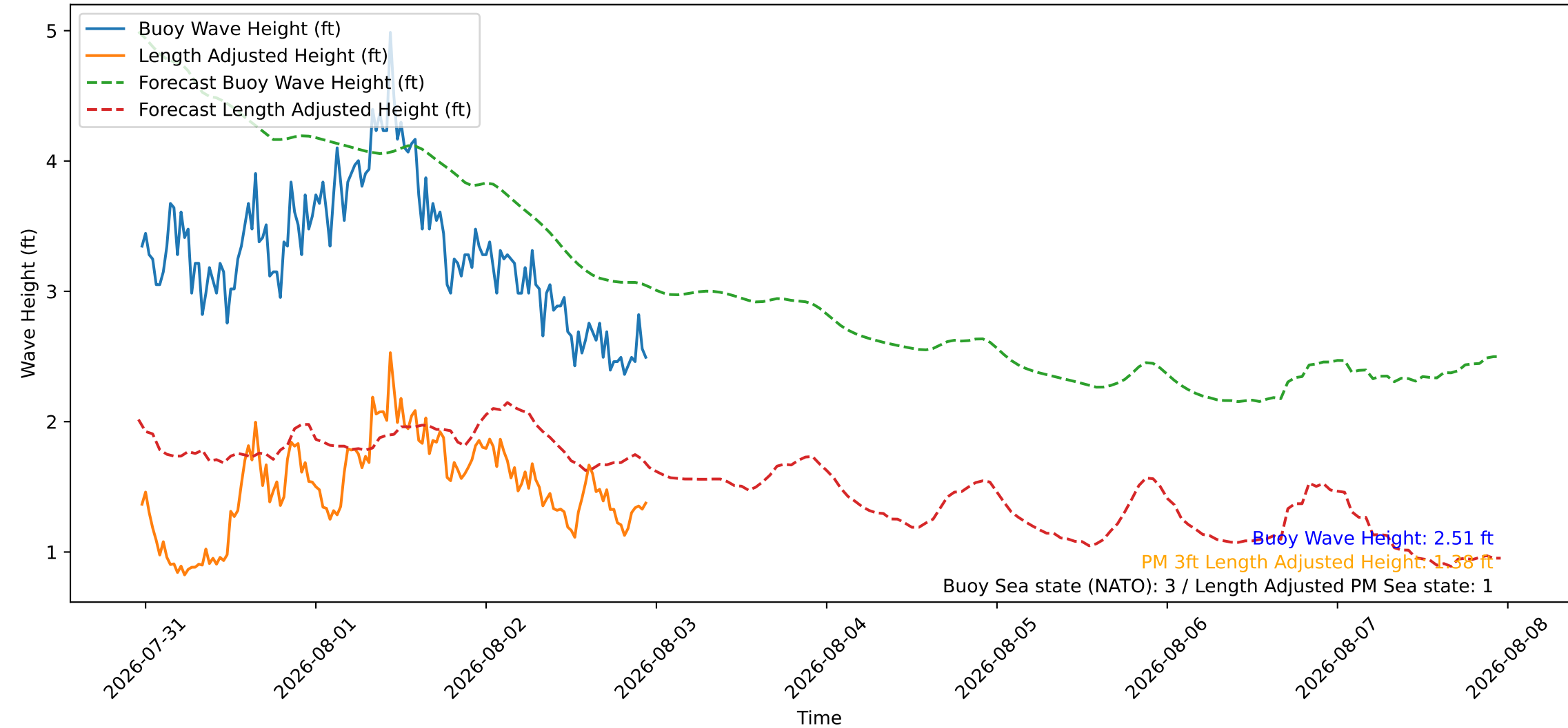
Wave Heights over Time for Green Beach at 2026-08-02 23:21:09
