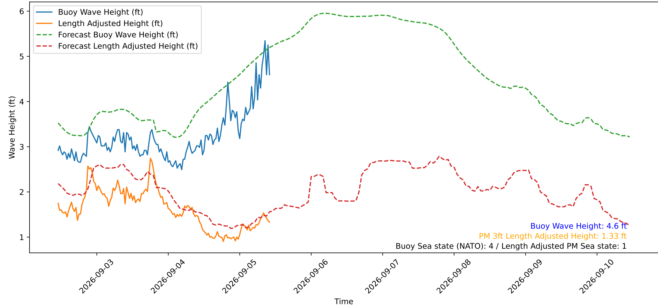
Wave Heights over Time for Green Beach at 2026-09-05 10:51:14
