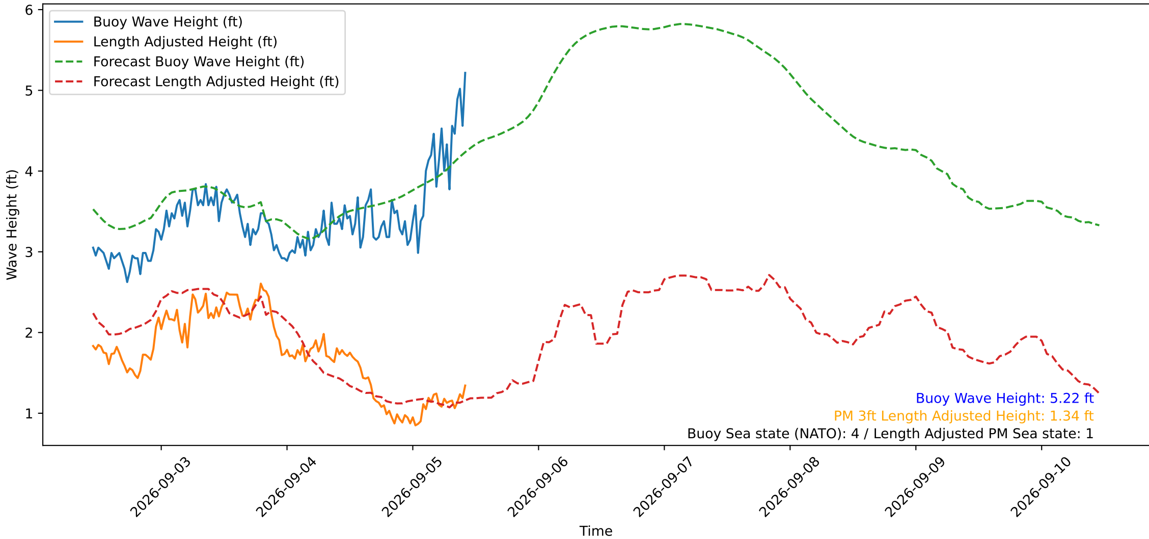
Wave Heights over Time for Oceanside Harbor at 2026-09-05 10:50:29
