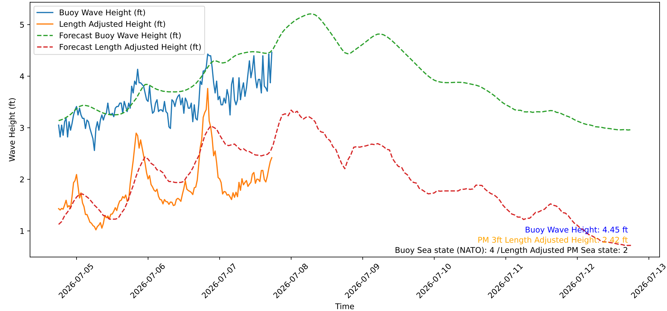
Wave Heights over Time for Green Beach at 2026-07-07 18:11:07
