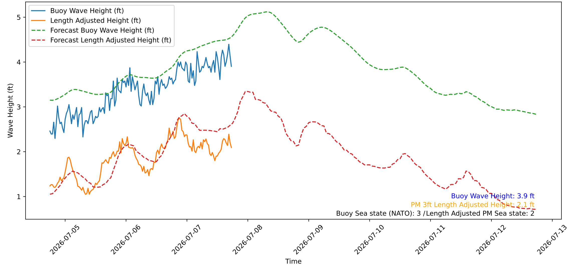
Wave Heights over Time for Oceanside Harbor at 2026-07-07 18:10:26
