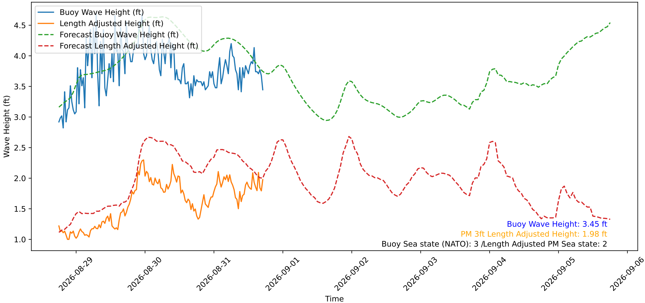
Wave Heights over Time for Red Beach at 2026-08-31 17:50:51
