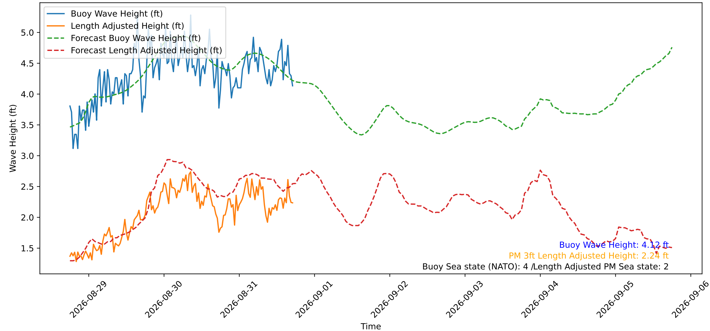
Wave Heights over Time for Oceanside Harbor at 2026-08-31 17:50:30
