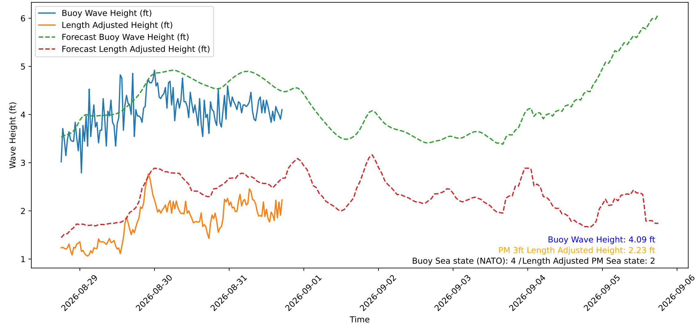
Wave Heights over Time for Green Beach at 2026-08-31 17:51:15
