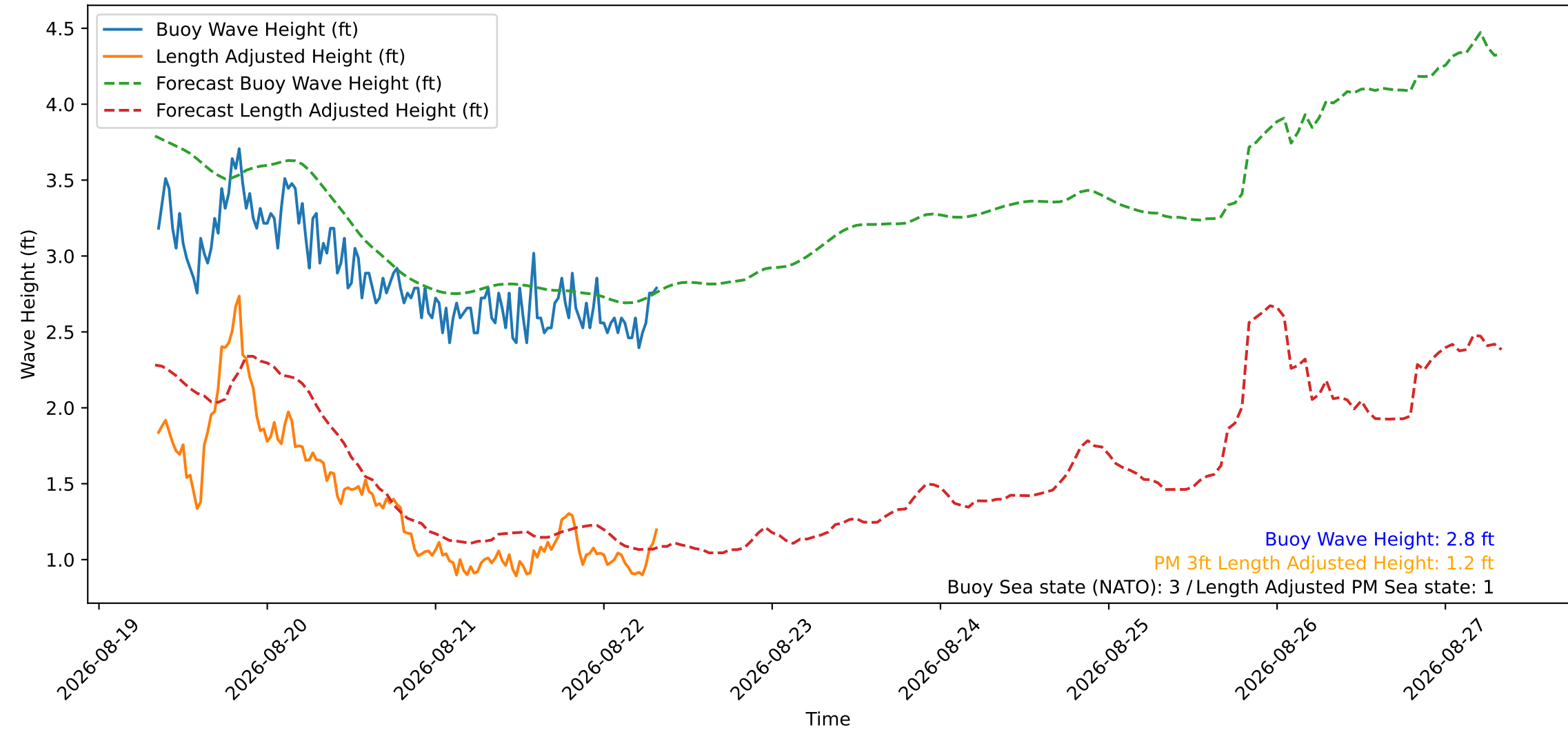
Wave Heights over Time for Green Beach at 2026-08-22 08:11:12
