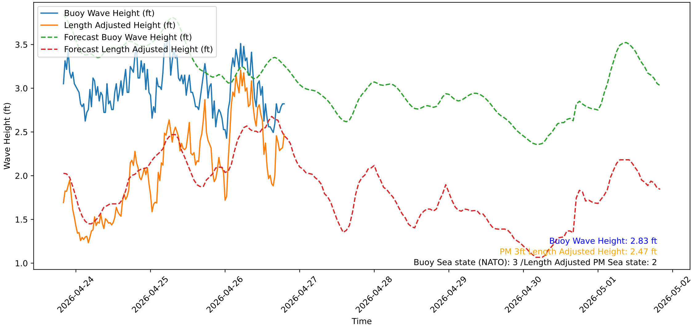
Wave Heights over Time for Green Beach at 2026-04-26 19:51:13
