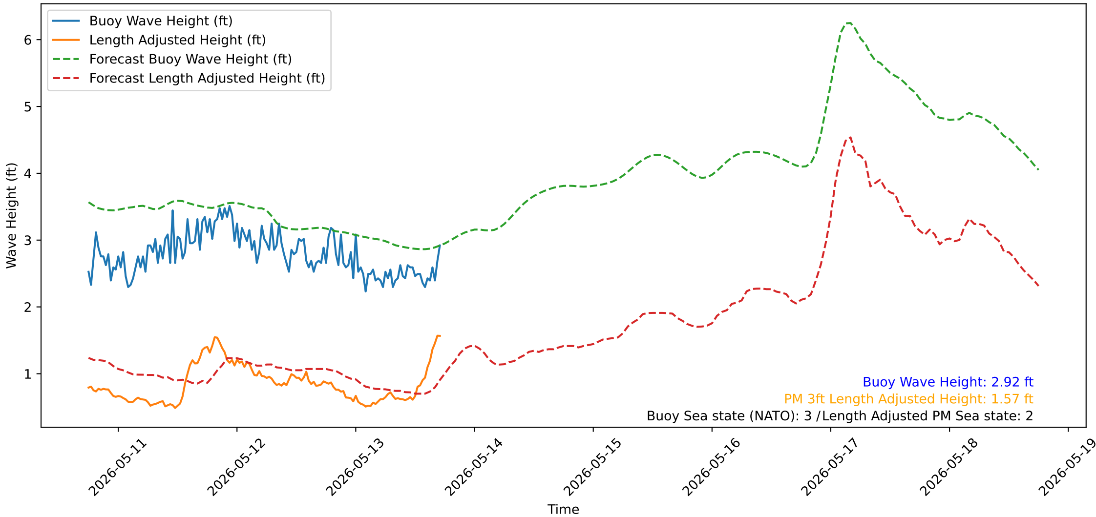
Wave Heights over Time for Green Beach at 2026-05-13 17:51:16
