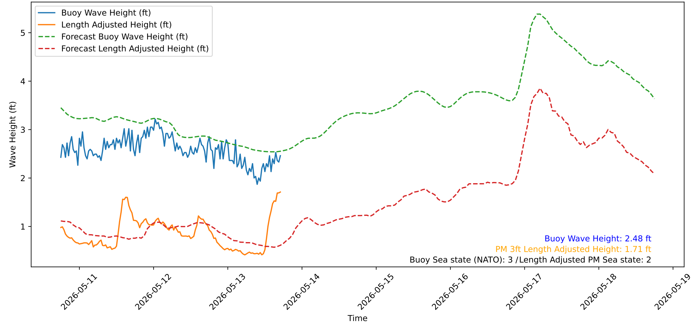
Wave Heights over Time for Red Beach at 2026-05-13 17:50:53
