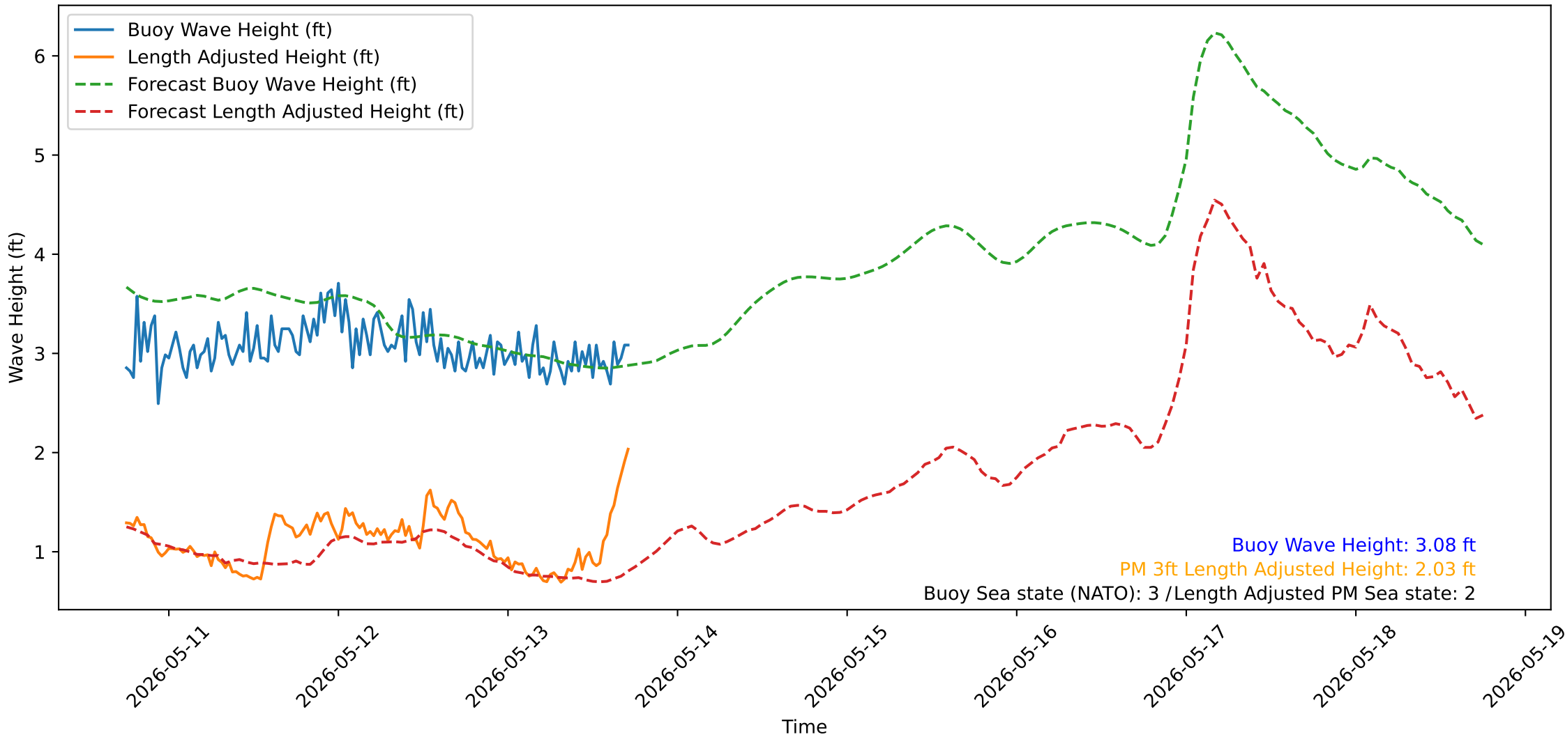
Wave Heights over Time for Oceanside Harbor at 2026-05-13 17:50:32
