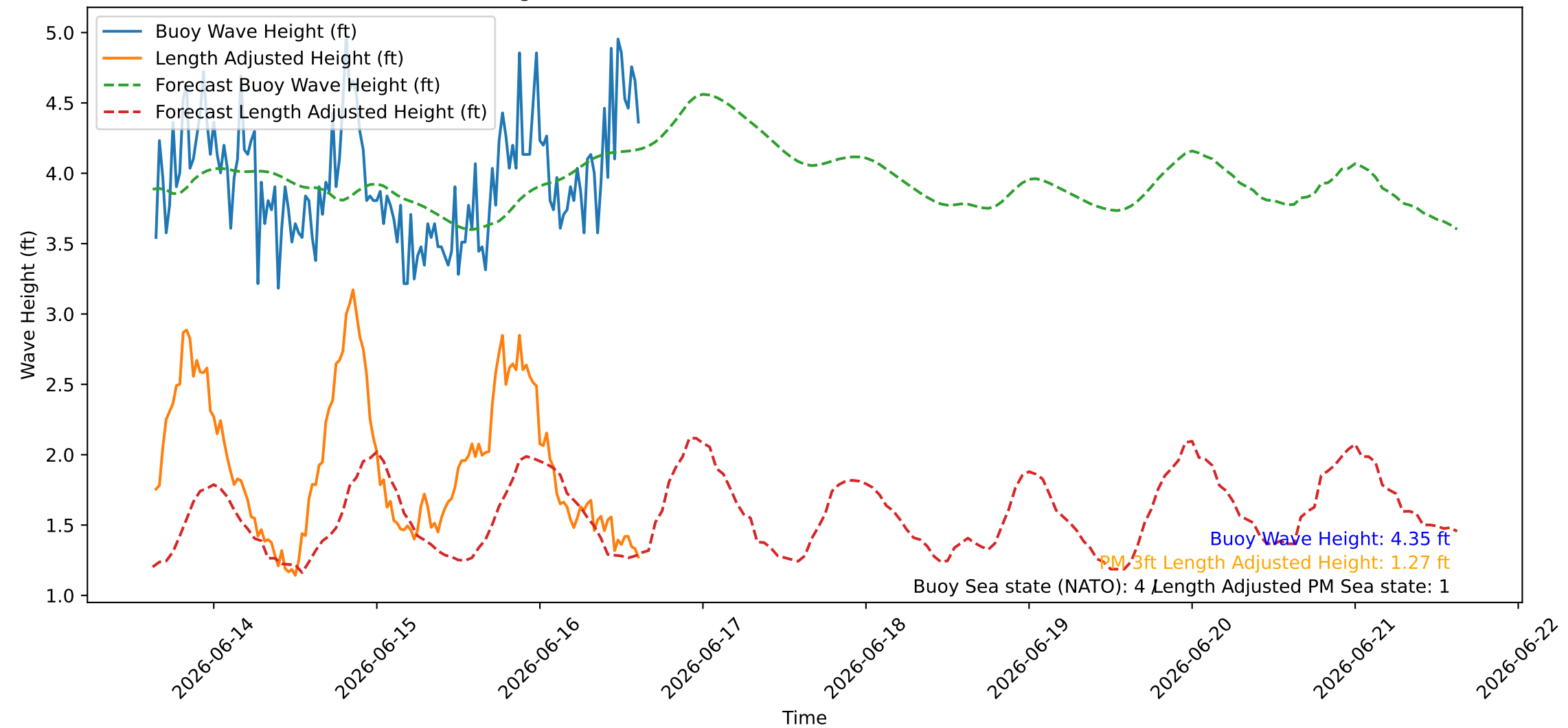
Wave Heights over Time for Oceanside Harbor at 2026-06-16 15:20:26
