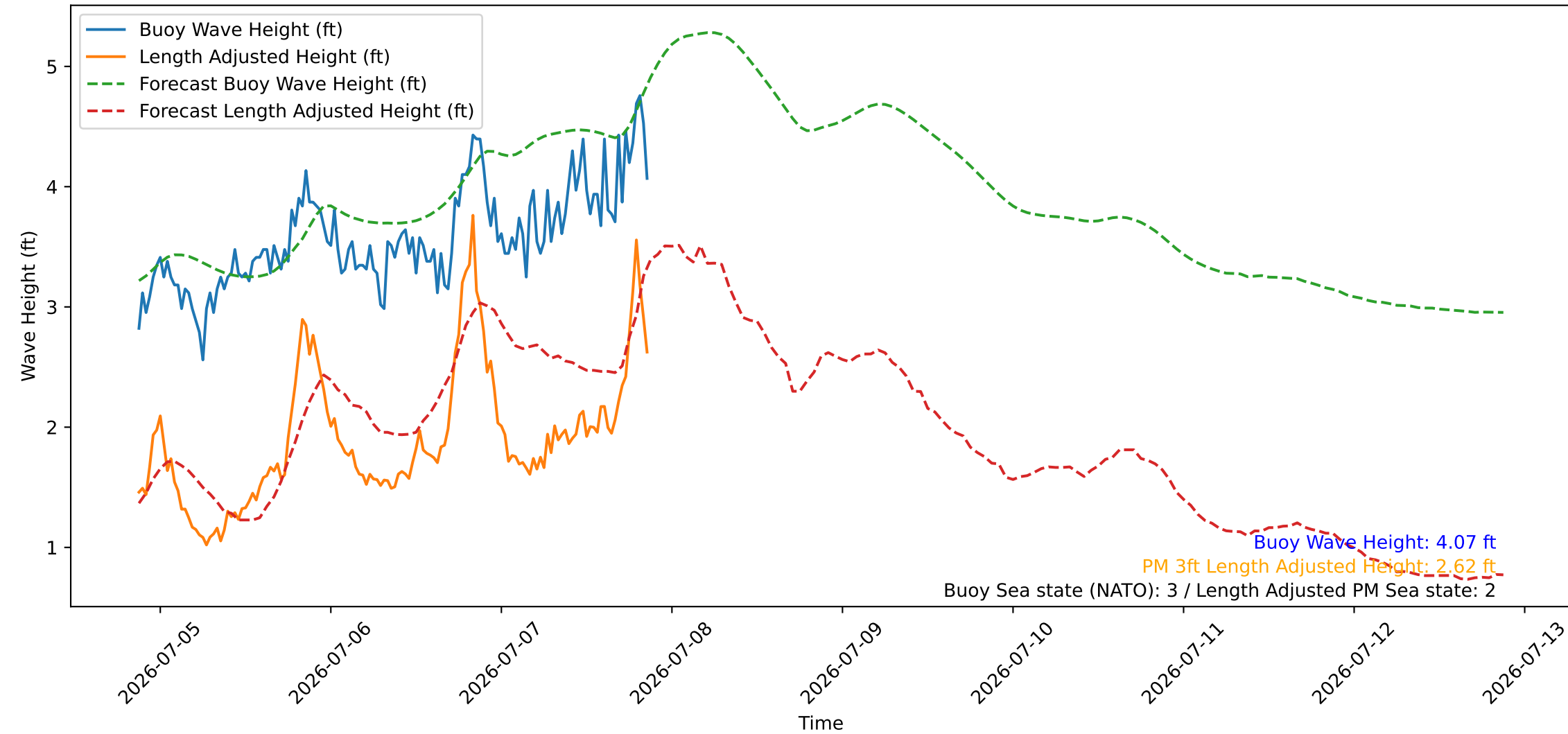
Wave Heights over Time for Green Beach at 2026-07-07 21:11:08
