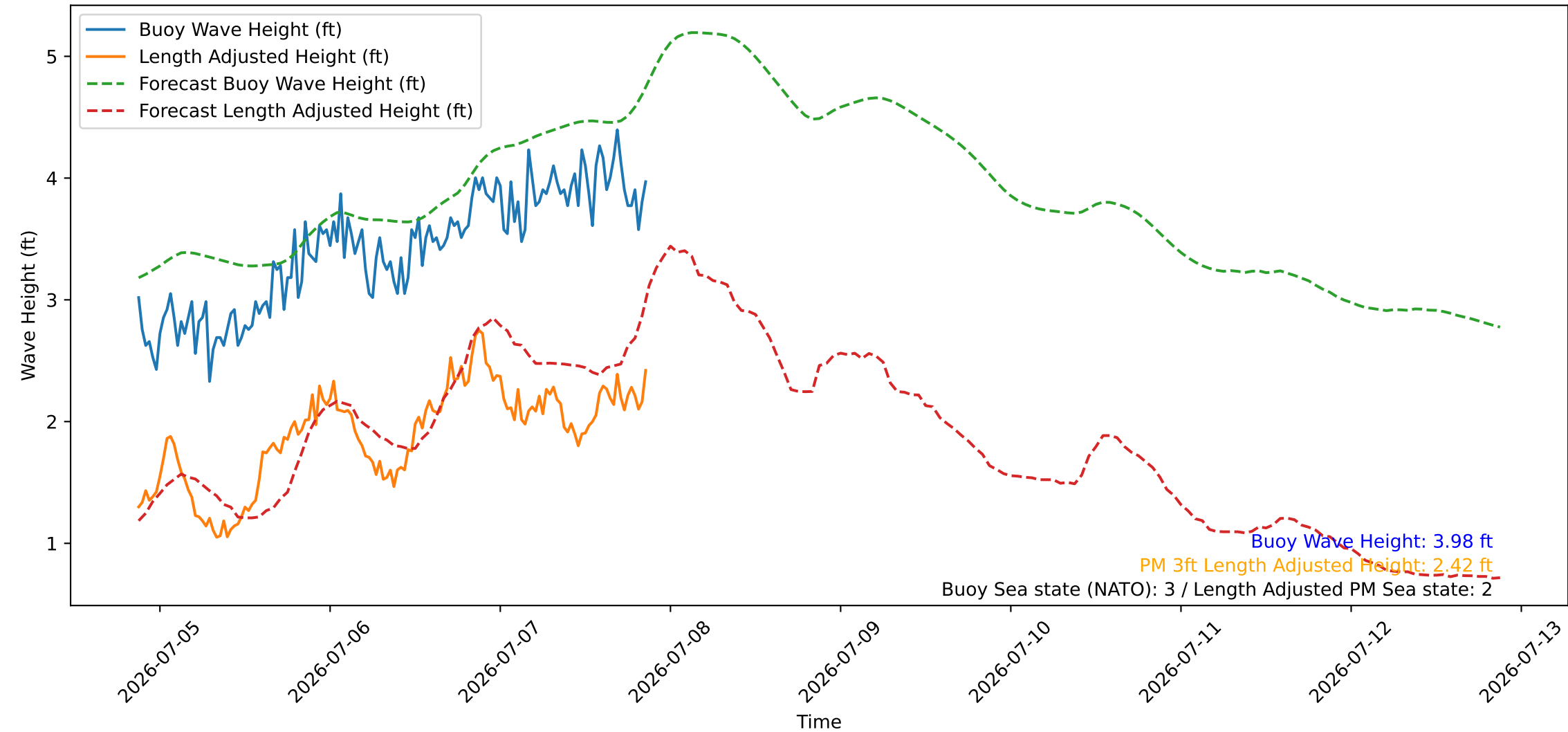
Wave Heights over Time for Oceanside Harbor at 2026-07-07 21:10:26
