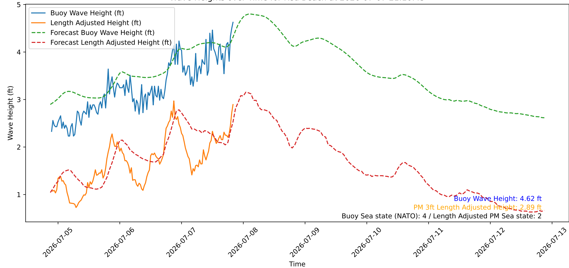
Wave Heights over Time for Red Beach at 2026-07-07 21:10:45
